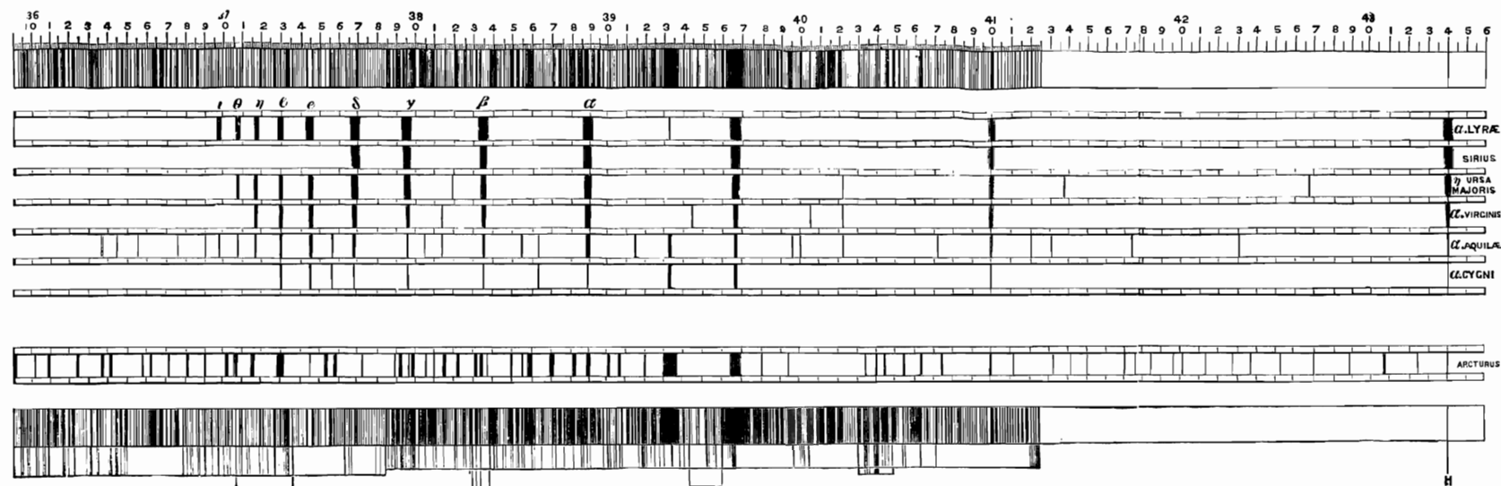
Map of Photographic Spectra of Seven Stars.
