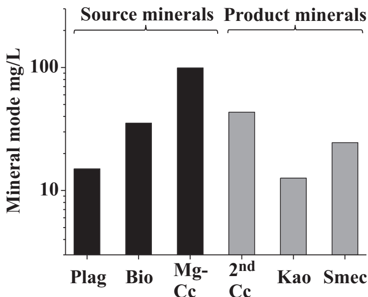
Fig. 18. Average mineral modes in mg/L calculated against bedload AK16 (AK145M gives indistinguishable results) using Mg/Ca for primary carbonate from acetic leach. Note that \sim 50\% of carbonate is re-precipitated as secondary calcite. If Mg/Ca from acetic plus HCl leaches is used for the primary carbonate, mineral mode mass balance requires dissolution of extra Ca implying the inferred Mg/Ca ratio is higher than the ratio of the carbonate weathered. Plag = plagioclase, Bio = biotite, Chl = chlorite, Mg-Cc = primary Mg-bearing carbonate, 2 nd -Cc = secondary calcite, Kao = kaolinite, Smec = smectite.
