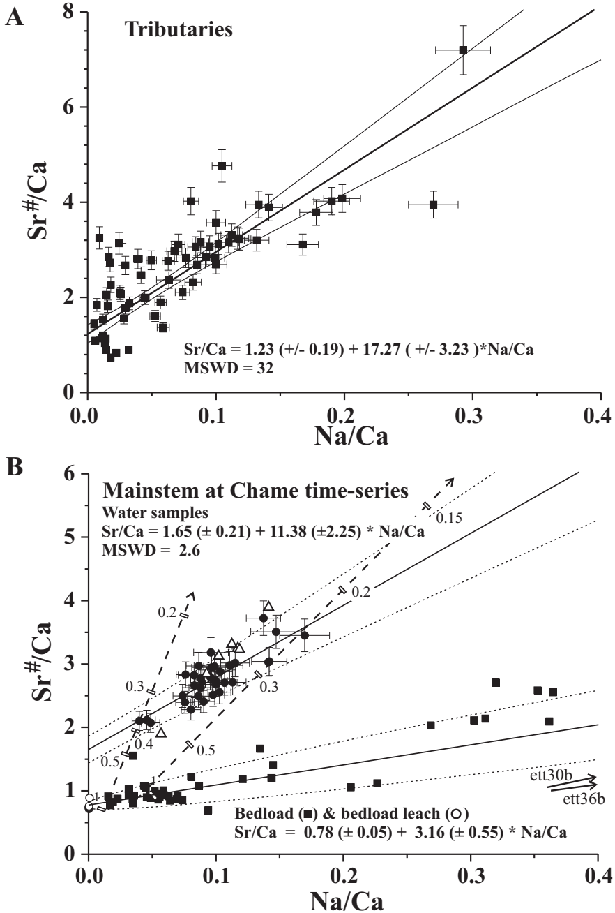
Fig. 5. (A) \text{Sr}^\#/\text{Ca} (mmol/mol) versus \text{Na}/\text{Ca} molar ratio correlation diagrams for water samples from May and September 2002 Marsyandi tributary sample sets. Line fit and 1\sigma uncertainties (dotted lines) as described by Bickle and others (2005). Error bars (not shown where smaller than symbols) are for 1\sigma and represent the combined uncertainties from the analyses and corrections for rain and hot-spring inputs. (B) \text{Sr}^\#/\text{Ca} (mmol/mol) versus \text{Na}/\text{Ca} molar ratio for time-series water samples from Marsyandi below Chame (circles with error bars) compared to bed-load (solid squares), and bed-load leaches (open circles). Open triangles are water samples from Marsyandi at and above Manang and Khangsar Khola. Best fits and 1\sigma error bounds (dotted lines) shown. 2 bed-load samples plot outside diagram. Dashed lines are trajectories showing loci of samples precipitating secondary calcite, assuming K_D \text{ Sr/Ca} = 0.05 (Rimstidt and others, 1998) for initial \text{Na}/\text{Ca} ratios of 0.015 and 0.04. Values are fraction of initial Ca remaining in water ( \gamma ).
