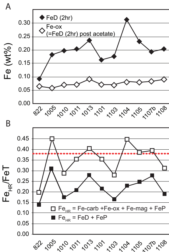
Fig. 11. (A) Dithionite-extractable iron (FeD) and dithionite-extractable iron extracted after an acetate extraction (Fe-ox). (B) \text{Fe}_{\text{HR}}/\text{FeT} in a subset of samples from the Walcott Quarry determined i) using the method of Raiswell and Canfield (1998), where \text{Fe}_{\text{HR}} is operationally defined as \text{FeD} + \text{FeP} , and ii) using the sequential extraction method of Poulton and Canfield (2005), where \text{Fe}_{\text{HR}} is operationally defined as \text{Fe-carb} + \text{Fe-ox} + \text{Fe-mag} + \text{FeP} .
