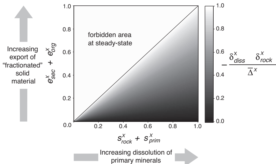
Fig. 3. Relative isotope difference \frac{\delta_{diss}^X - \delta_{rock}^X}{\bar{\Delta}^X} (eq 9) as a function of (s_{rock}^X + s_{prim}^X) (proportion of X dissolved at the weathering front and within the regolith) and (e_{sec}^X + e_{org}^X) (proportion of X exported as solid secondary weathering products or as solid organics). White corresponds to the highest difference in isotope composition observable between rock and dissolved compounds, at steady-state. In this case this difference is equal to the lumped isotope fractionation factor \bar{\Delta}^X (eq 7). Black corresponds to the case where there is no difference in isotope composition between rock and dissolved compounds. Note that the value on the Y-axis ( e_{sec}^X + e_{org}^X ) cannot exceed, at steady-state, that on the X-axis ( s_{rock}^X + s_{prim}^X ), since X needs to be unlocked from primary minerals before being incorporated (and hence undergo isotope fractionation) into solid secondary weathering products or into organic matter. This condition implies the existence of a “forbidden area”.
