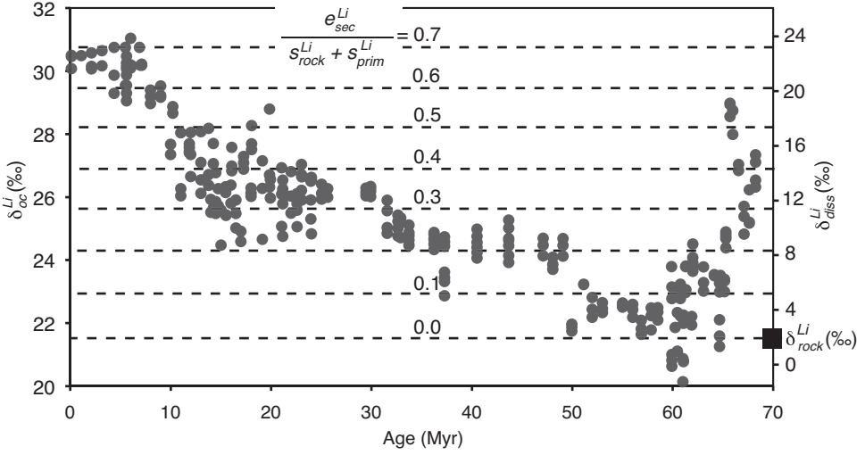
Fig. 8. Li stable isotope record in the ocean from Misra and Froelich (2012) and weathering conditions on the continents through the Cenozoic. All parameters are represented by the same set of data points, only axes change, since the different parameters are linearly related. Left axis: Li isotope composition for the oceans ( \delta_{oc}^{Li} ) as measured in foraminifera (Misra and Froelich, 2012). Right axis: corresponding values for Li isotope composition of the global river dissolved load ( \delta_{diss}^{Li} ) derived from an ocean mass-balance (Appendix D; Misra and Froelich, 2012). Stippled lines: corresponding value of the ratio between Li export as secondary weathering products ( e_{sec}^{Li} ) and Li released from primary minerals ( s_{rock}^{Li} + s_{prim}^{Li} ), calculated following equation (11), and assuming that \delta_{diss}^{Li} from the ocean mass-balance is equivalent to \delta_{diss}^{Li} of the model.
