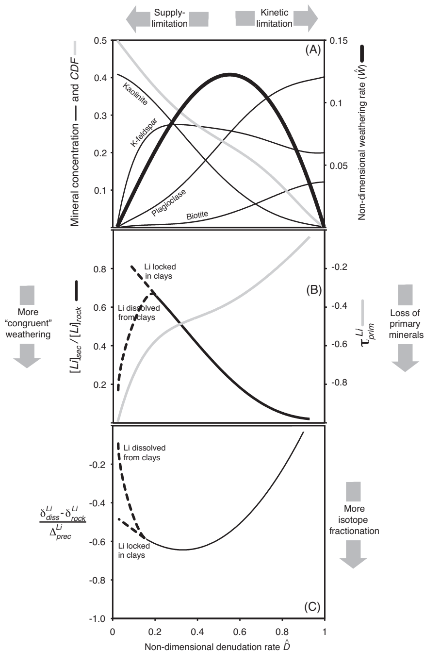
Fig. 9. Modeling of Li behavior in the global weathering zone following the results of Ferrier and Kirchner (2008) (panel A). The bedrock has a granitic composition (quartz is not shown). Non-dimensional denudation rate \hat{D} is the denudation rate D normalized to the maximum soil production rate obtained for an infinitely thin regolith. At high denudation rates, regolith residence time is short and weathering intensities (as shown by CDF ) and rates (non-dimensional weathering rate \hat{W} that is W normalized to the maximum soil production rate) are low: the system is kinetically-limited . At low denudation rates, regolith residence time is long and weathering intensities are high: CDF reaches a value of 0.5, and weathering of biotite, plagioclase and K-feldspar run to completion, whereas the maximum amount of precipitated kaolinite is reached.
