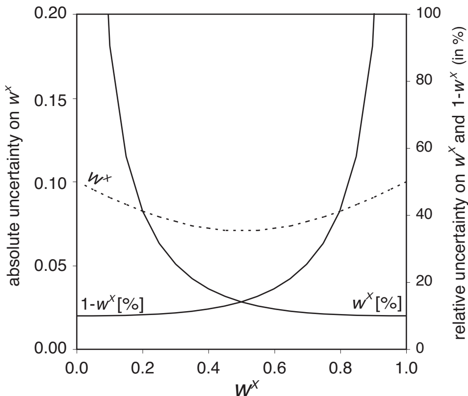
Fig. 7. Absolute (stippled line) and relative (solid lines) uncertainties on the proportion of dissolved export of X , w^X , and the proportion of particulate export, 1 - w^X , calculated from isotope compositions of river material (dissolved and particulate) and source rock, as a function of w^X . The absolute uncertainty in w^X is identical to that in 1 - w^X . Details of the calculations and hypotheses are given in Appendix B. Uncertainty on source rock isotope composition \delta_{rock}^X was assumed to be 0. Important parameters of this uncertainty propagation (Appendix B) are the ratios between (1) the uncertainty on \delta_{diss}^X and on \delta_{sed}^X ; (2) the difference (\delta_{sed}^X - \delta_{diss}^X) . Here these ratios are equal to 0.1, following data reported in the literature for small river on Mg and Li isotopes. This figure is thought to be representative of the uncertainties to be encountered at the small river scale, although uncertainties on the source isotope composition ( \delta_{rock}^X ) would uniformly shift the uncertainty curves towards higher values.
