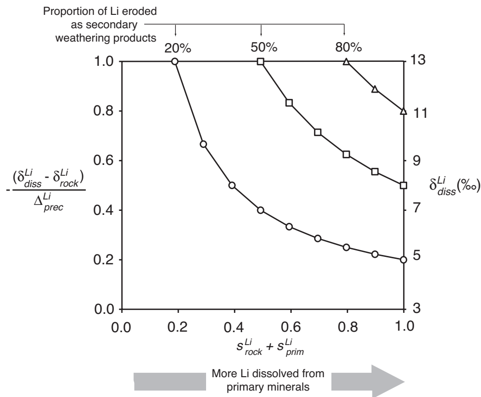
Fig. 5. Relative isotope fractionation of Li (eq 11) as a function of s_{rock}^{Li} + s_{prim}^{Li} (proportion of Li released from primary minerals, X-axis), for 3 different proportions of Li exported as secondary weathering products ( e_{rock}^{Li} upper labels). On the right Y-axis, the resulting isotope composition of soil water is indicated, assuming \delta_{rock}^{Li} of 3‰ and \Delta_{prec}^{Li} of -10 ‰.
