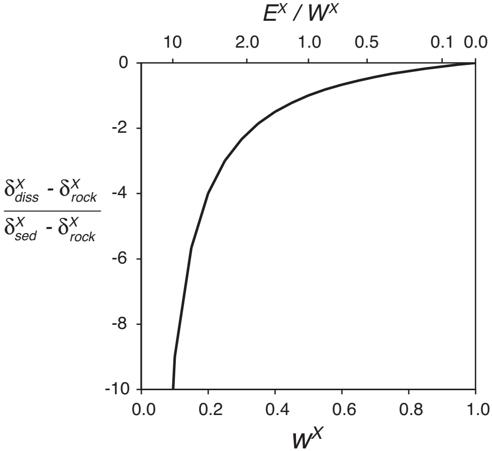
Fig. 6. Ratio of the differences in isotope composition between a dissolved element in soil water or river water and bedrock, to that between the same element in river sediment or topsoil and bedrock, as a function of the fraction of dissolved export w^X (lower X-axis) and the ratio of the elemental erosion flux E^X to the weathering flux W^X (upper X-axis).
