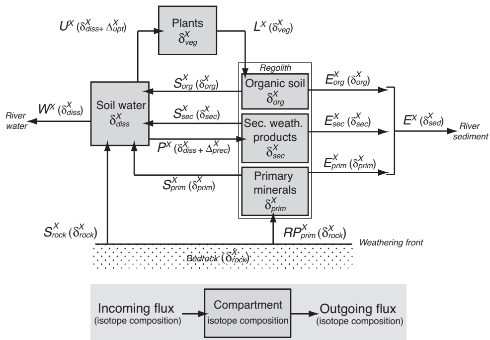
Fig. 1. Schematic diagram of the weathering zone model. See text and table 1 for symbols.
