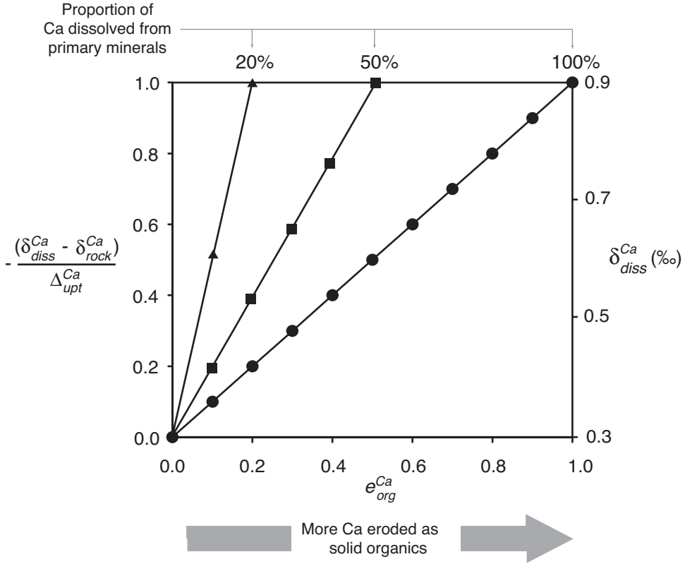
Fig. 4. Relative isotope fractionation of Ca (eq 10) as a function of e_{org}^{Ca} (proportion of Ca exported as solid organic, X-axis), for 3 different proportions of Ca released from primary minerals ( s_{rock}^{Ca} + s_{prim}^{Ca} , upper X-axis labels). On the right Y-axis, the resulting isotope composition of soil water is indicated, assuming \delta_{rock}^{Ca} of 0.3‰ and \Delta_{upt}^{Ca} of -0.6‰.
