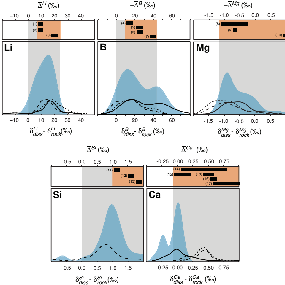
Fig. 2. Distributions (probability density functions) of isotope composition of soil water, ground water, and river water (large panels, \delta_{diss}^X and \delta_{diss}^X - \delta_{rock}^X ) and weathering-related isotope fractionation factors (small panels, -\Delta^X and -\Delta_{upt}^X ) compiled from the literature, for the novel stable isotope systems \delta^7\text{Li} , \delta^{11}\text{B} , \delta^{26}\text{Mg} , \delta^{30}\text{Si} , and \delta^{44/42}\text{Ca} (Appendix B). Large panels: color-filled blue curves are distributions of (\delta_{diss}^X - \delta_{rock}^X) data corrected for “external inputs” (rain, dust, and anthropogenic inputs and evaporite weathering). These curves thus reflect silicate weathering for B, Li and Si, and both silicate and carbonate weathering for Ca and Mg. As both corrections for external inputs and estimates of \delta_{rock}^X introduce significant uncertainties (Appendix B), also plotted for comparison are non-corrected \delta_{diss}^X data (dotted curves), external inputs-corrected \delta_{diss}^X data (stippled curves) and non-corrected (\delta_{diss}^X - \delta_{rock}^X) data (solid curves). In these diagrams, the vertical scale is arbitrary. Small panels: range of published isotope fractionation factors (1) co-precipitation of Li into calcite at 5 to 30 °C (Mariott and others, 2004); (2) incorporation of Li into smectite at 25 to 90 °C (Vigier and others, 2008); (3) incorporation of Li into basalt during seafloor weathering (Chan and others, 1992); (4) adsorption of B onto birnessite at 25 °C, pH < 8 (Lemarchand and others, 2007); (5) adsorption of B onto Mississippi sediment (Spivack and others, 1987); (6) adsorption of B onto humic acids at 25 °C, 5 < pH < 9 (Lemarchand and others, 2005); (7) adsorption of B onto goethite at 25 °C, pH < 8 (Lemarchand and others, 2005); (8) uptake of Mg by rye grass and clover (Bolou-Bi and others, 2010); (9) uptake of Mg by wheat (Black and others, 2008); (10) co-precipitation of Mg into calcite at 26.5 °C (Saulnier and others, 2012); adsorption of Si onto (11) goethite and (12) ferrihydrite (Delstanche and others, 2009); (13) uptake of Si by bamboo (Ding and others, 2009); (14) precipitation of Ca as calcite at 25 °C, rate-dependent (DePaolo, 2011); adsorption of Ca onto (15) montmorillonite, (16) illite, and (17) kaolinite in seawater at 21 °C (Ockert and others, 2013); (18) uptake of Ca by beans (Cobert and others, 2011). Importantly, these isotope fractionation factors are not derived from field studies on continental weathering studies, such that there is no redundancy of data between the large and the small panels. For each of the isotope system, the best estimate of the lumped isotope fractionation factor -\Delta^X lies in the range defined by these process-specific fractionation factors, and is given by the orange area. The light gray area extending over both small and large panels is the range of (\delta_{diss}^X - \delta_{rock}^X) values predicted by our model (eq 9), that is between 0 and -\Delta^X .
