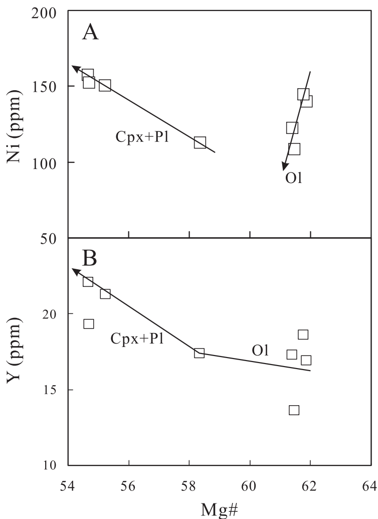
Fig. 8. Plots of (A) Ni vs. Mg# and (B) Y vs. Mg# showing that the Zhenzhushan basalts underwent fractional crystallization of olivine first and then clinopyroxene and plagioclase. Symbols are as in figure 4.
