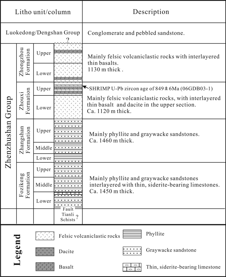
Fig. 2. Stratigraphic column of the Zhenzhushan Group in northeastern Jiangxi, South China (after Deng and others, 2003).
