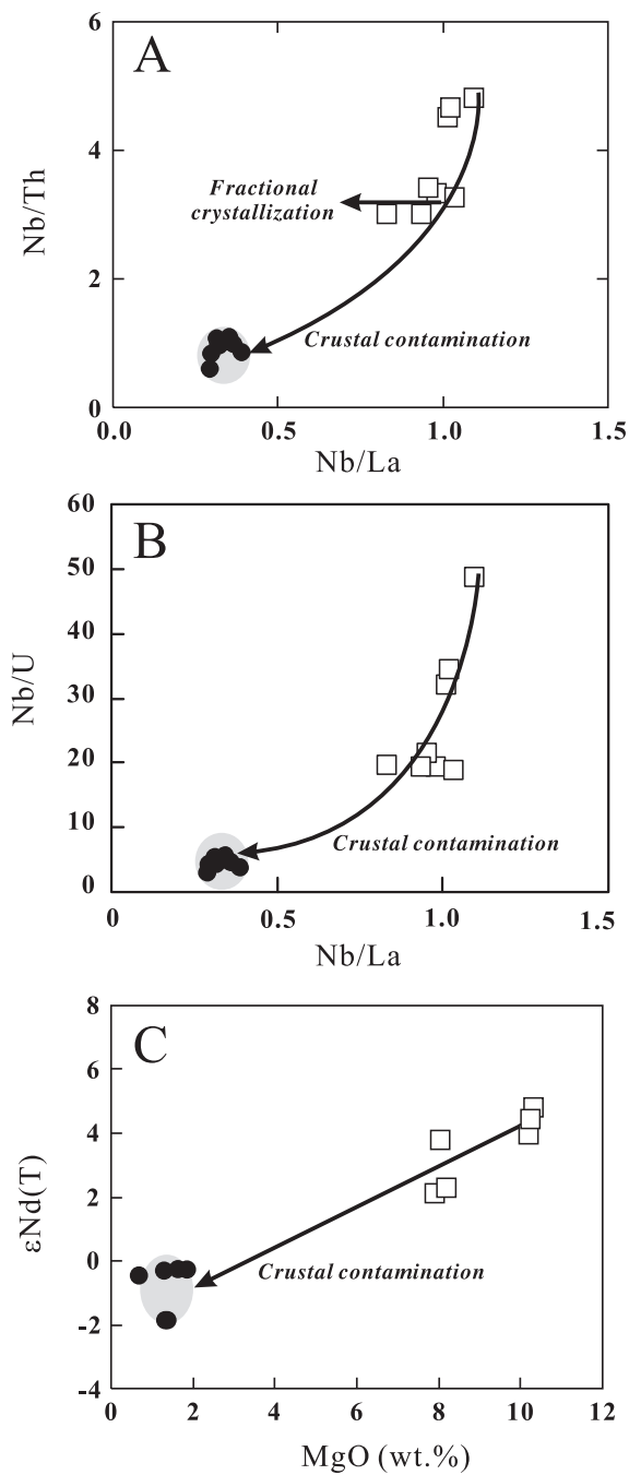
Fig. 9. Plots of (A) Nb/Th vs. Nb/La, (B) Nb/U vs. Nb/La and (C) \epsilon\text{Nd(T)} vs. MgO showing trends of contamination by crustal materials (possibly associated felsic volcanic rocks). Symbols are as in figure 4.
