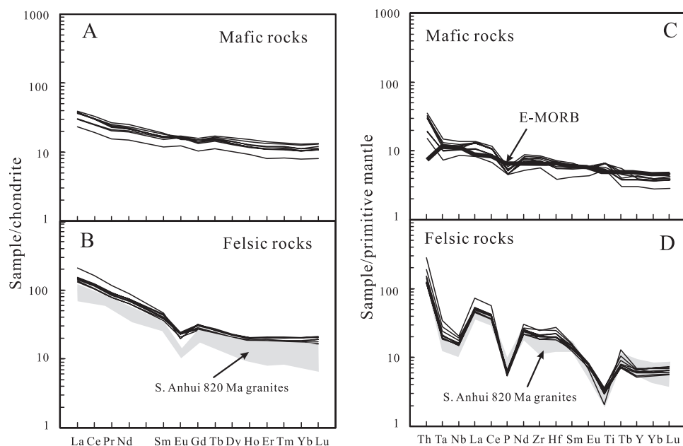
Fig. 7. Chondrite-normalized REE diagrams (A, B) and primitive mantle-normalized trace element diagrams (C, D) for the Zhenzhushan volcanic rocks. The data for the ca. 820 Ma southern Anhui granites are from X. H. Li and others (2003a). Normalization values are from Sun and McDonough (1989).
