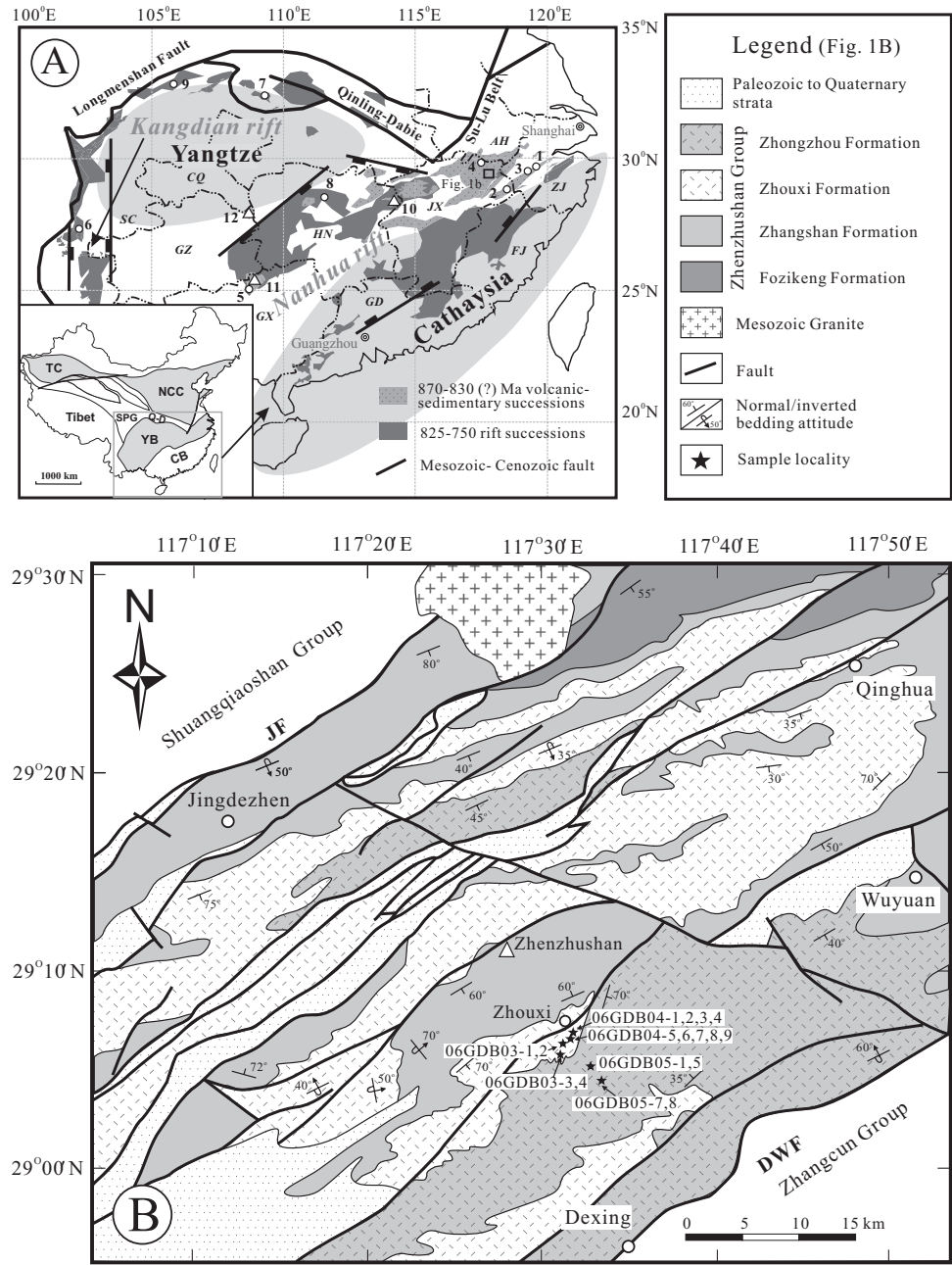
Fig. 1. (A) Distribution of mid-Neoproterozoic volcanic-sedimentary rocks and rift basins in the South China Block. DWF: Dexiong-Wuyuan Fault; JF: Jingdezhen Fault. Source of information: 1— 838 \pm 5 Ma Chencai bimodal volcanic rocks and 841 \pm 6 Ma Lipu diorite (Z. X. Li and others, 2010); 2— 848 \pm 4 Ma Ganbian syenitic complex (X. H. Li and others, 2010); 3— 849 \pm 7 Ma Shenwu doleritic dyke (X. H. Li and others, 2008); 4— \leq 770 Ma Shuangqiaoshan quartz-keratophyres (X. L. Wang and others, 2008; X. H. Li and others, 2009a); 5— 836 \pm 3 Ma Zhaigun granodiorite (X. L. Wang and others, 2006); 6— 857 \pm 13 Ma Guandaoshan diorite (X. H. Li and others, 2003b; Sun and Zhou, 2008); 7— 844 \pm 2 Ma Fangcheng syenite (Bao and others, 2008); 8— 823 \pm 6 Ma Yiyang Komatiitic basalt (X. C. Wang and others, 2007); 9— 820\text{--}810 Ma Bikou continental flood basalts (X. C. Wang and others, 2008); 10—ca. 860 Ma detrital zircons in the Lengjiayi Formation (X. L. Wang and others, 2007); 11— 860\text{--}870 Ma detrital zircons in the
