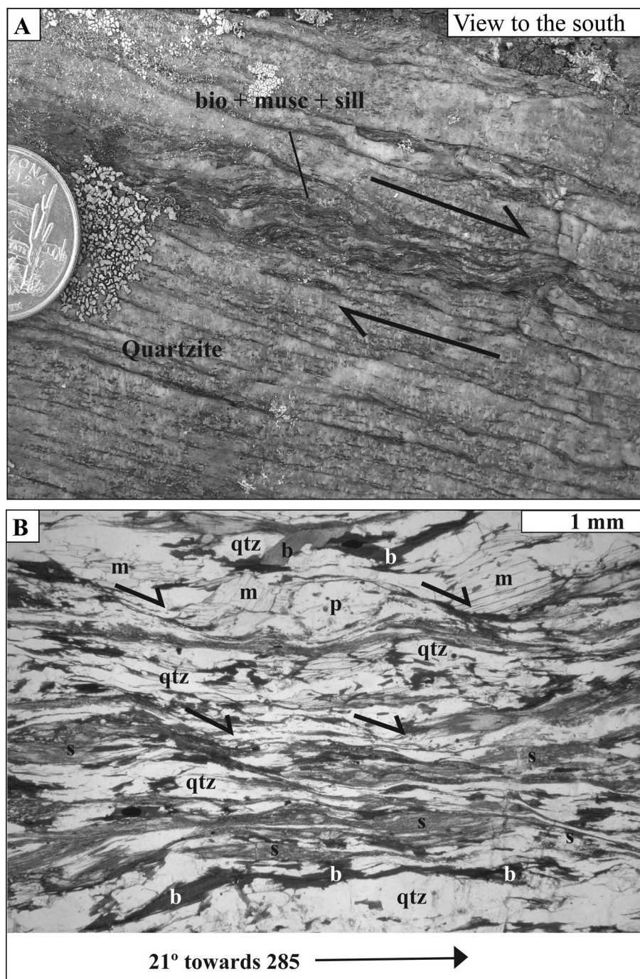
Fig. 5. High-grade fabrics in the country rock the Middle Mountain gneiss. (A) Vertical cliff face of quartzite with aluminous horizons. Edge of quarter for scale (field of view \sim 8 cm wide), view to the south; the cliff face is roughly parallel to the gently west-dipping stretching lineation. Asymmetry in fabric indicates down-to-the-west sense of shear. (B) The aluminous horizon in plain polarized light shows the fabric is defined by fibrolitic sillimanite (s; abundant fine gray fibrous), biotite (bio), muscovite (m), and quartz ribbons (qtz). Shear bands indicating top-to-the-west-sense of motion and indicated by black arrows.
