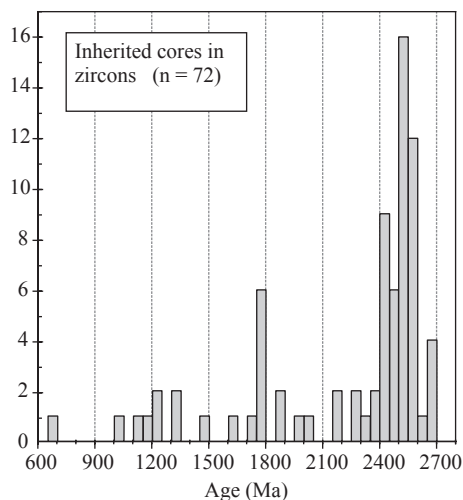
Fig. 7. Histogram of ^{204}\text{Pb} -corrected ^{207}\text{Pb}/^{206}\text{Pb} ages of inherited cores from the zircons of the Cassia plutonic complex including those reported for the Red Butte pluton by Egger and others (2003). The ages are dominantly 2.4–2.7 Ga. A second, smaller peak of ages near ca. 1.8 Ga may reflect known orogenic events, such as the Trans Hudson orogeny or Medicine Bow orogeny. The youngest core analyzed is 697 \pm 7 Ma.
