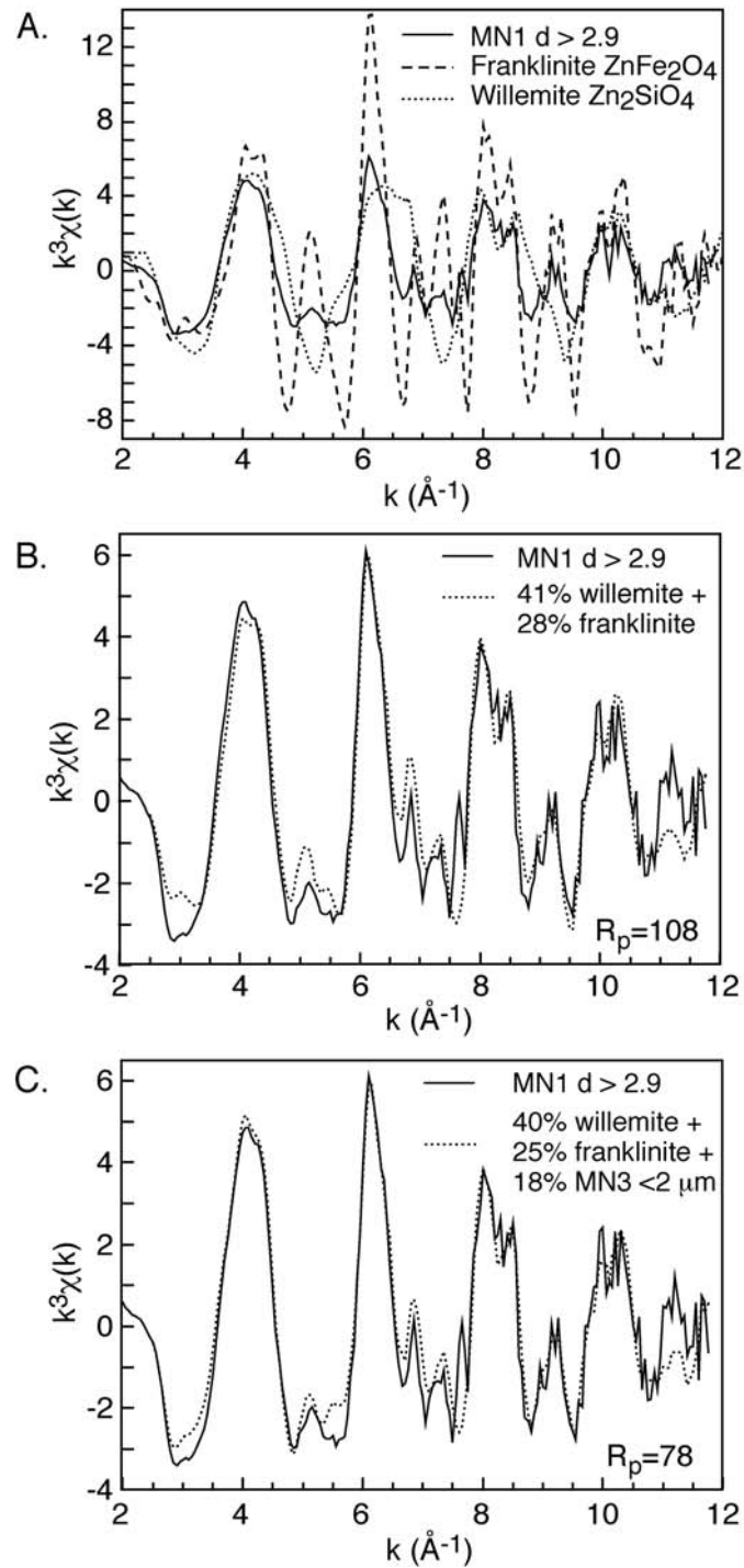
Fig. 7(A) Zn K-edge EXAFS of the dense fraction ( d > 2.9 ) of MN1 together with franklinite and willemite. (B) Optimal 2-component model of MN1 d > 2.9 assuming 28 percent franklinite + 41 percent willemite. (C) Optimal 3-component model of MN1 d > 2.9 assuming 25 percent franklinite + 40 percent willemite + 18 percent MN3 < 2 \mu\text{m} fraction.
