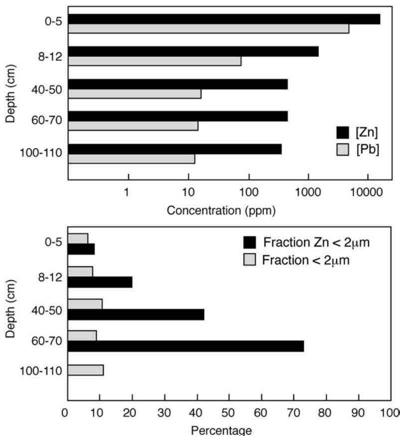
Fig. 5(A) Profile concentration of Zn and Pb in the silt fraction (<100 μm) of the soil from Mortagne du Nord (samples MN1-MN5). (B) Relative distribution of Zn in the clay fraction (<2 μm) and percentage of the clay fraction in the <2 mm soil fraction. Zn is increasingly concentrated in the clay fraction with depth.
