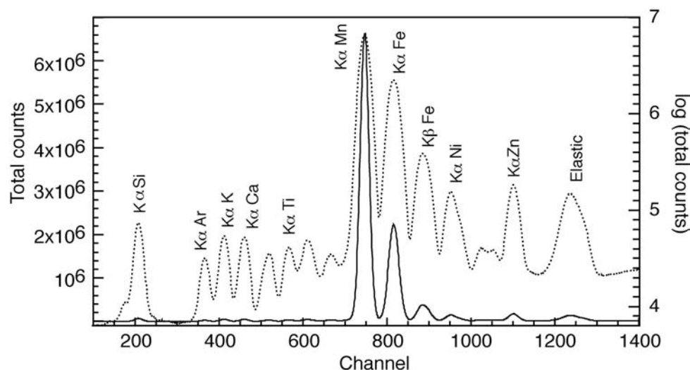
Fig. 3. Energy dispersive X-ray (EDX) spectrum recorded at 10 keV and integrated during the 8 h of acquisition time of elemental maps presented in figure 18B. The total signal is heavily dominated by the Fe and Mn fluorescence-yield of the soil matrix, the Zn signal making only \sim 2 \cdot 10^5 counts.
