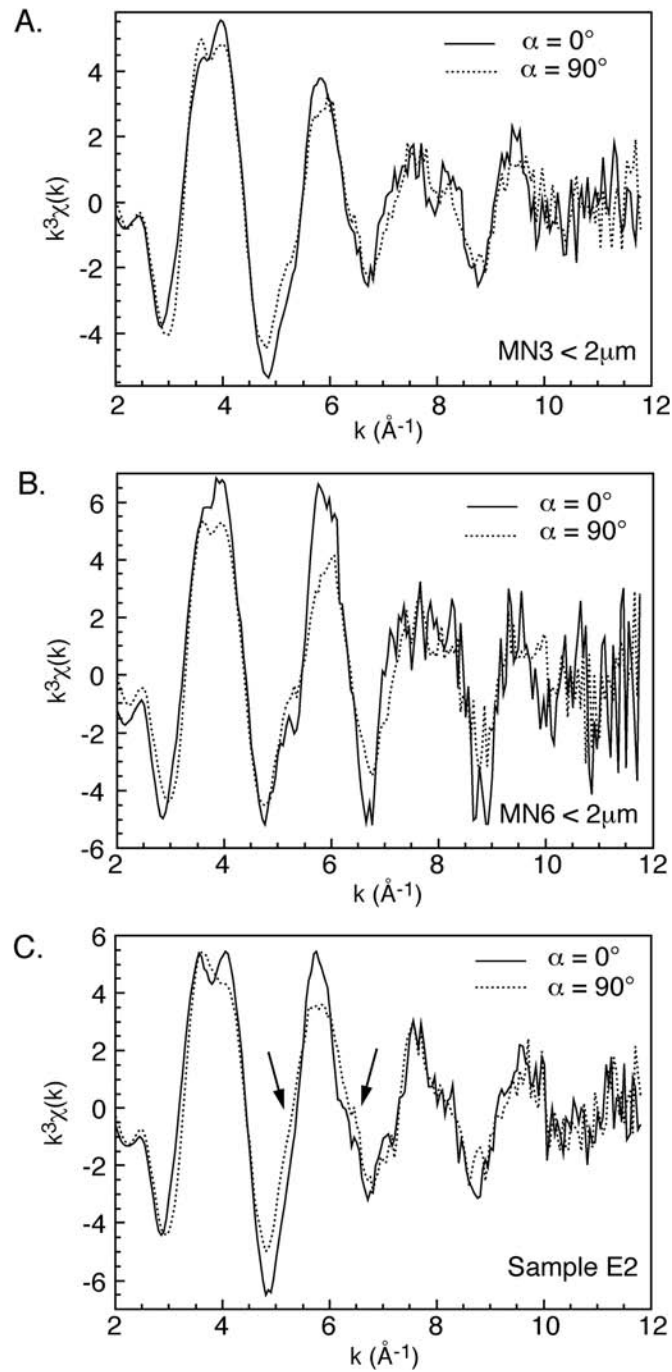
Fig. 15. In-plane ( \alpha = 0^\circ ) and out-of-plane ( \alpha = 90^\circ ) Zn K-edge P-EXAFS spectra of MN3 < 2 \mu\text{m} (A), MN6 < 2 \mu\text{m} (B), and E2 (C).
