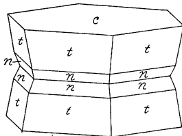
FIGS. 2, 3, 4.—Crystals of \text{SrO.SiO}_2 .
