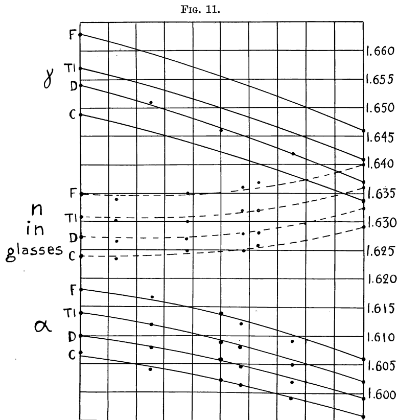
FIG. 11.—Variation of the indices of refraction in the mix crystal series \text{CaO.SiO}_2\text{-SrO.SiO}_2 .
