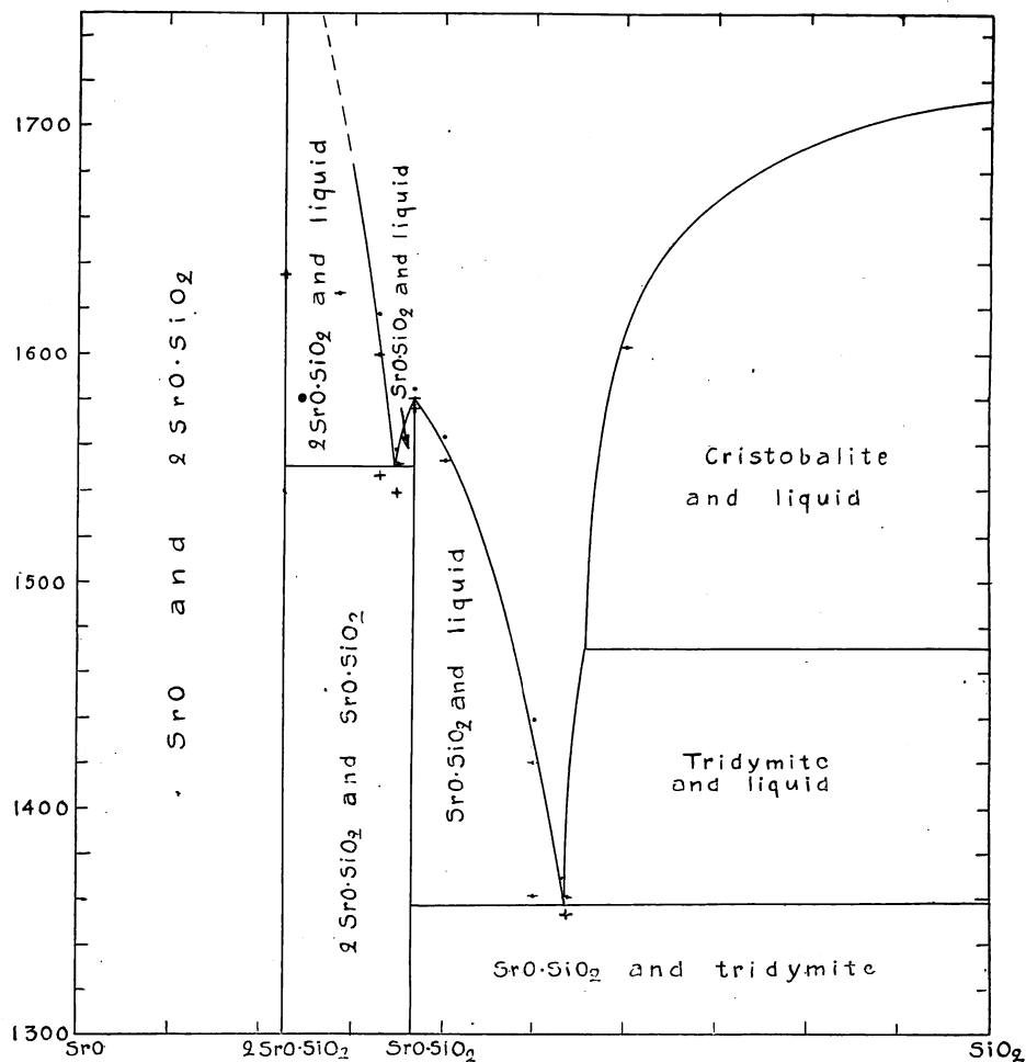
—Fig. 1.—Temperature-concentration diagram of the binary system \text{SrO-SiO}_2 .
