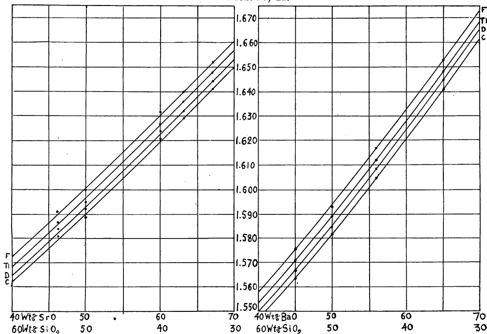
Fig. 13.—Variation of the indices of refraction in strontium silicate glasses.
