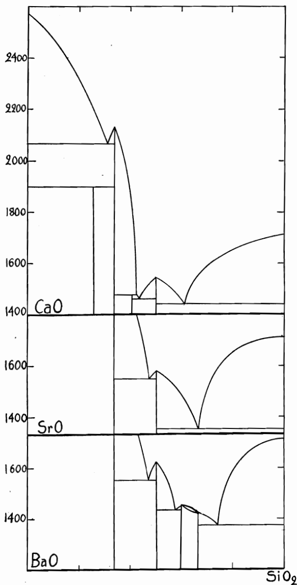
FIG. 17.—Synopsis of the binary systems \text{BaO-SiO}_2 , \text{SrO-SiO}_2 , and \text{CaO-SiO}_2 in mol. %.
