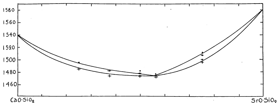
FIG. 10.—Temperature-concentration diagram of the binary system \text{CaO}.\text{SiO}_2\text{--SrO}.\text{SiO}_2 showing a complete series of mix crystals with a minimum.
