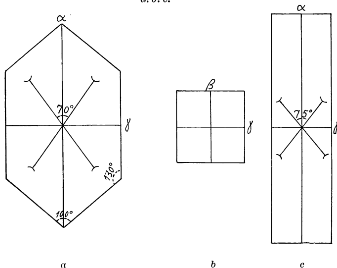
FIG. 8.—Optical orientation in crystals of barium disilicate: \alpha = crystals in optical glass after N. L. Bowen; b and c = crystals from \text{BaCl}_2 -flux, and as formed in barium silicate melt.
