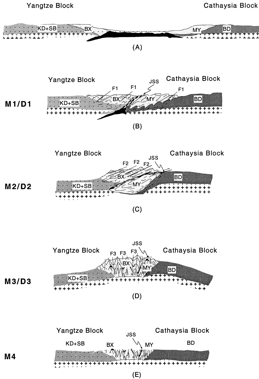
Fig. 13. A series of schematic sections showing the suggested tectonothermal evolution for assembly of the Cathaysia and Yangtze blocks. Abbreviation: BD-Badu assemblage; BX-Banxi assemblage; JSS-Jiangshan-Shaoxing suture; KD-Kangding assemblage; MY-Mayuan assemblage; SB-Sibao assemblage.
