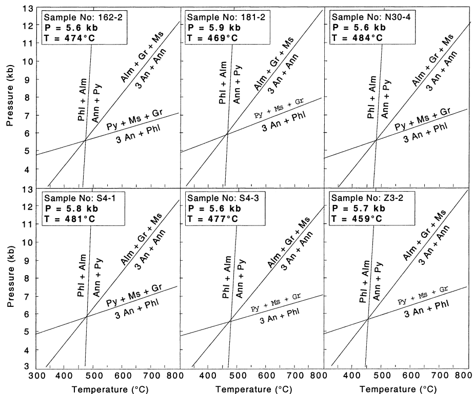
Fig. 8. P-T estimates for the M_1 stage computed by simultaneous solution of the garnet-biotite thermometer and the garnet-muscovite-biotite-plagioclase barometer using the TWEQU software package of Berman (1991).
