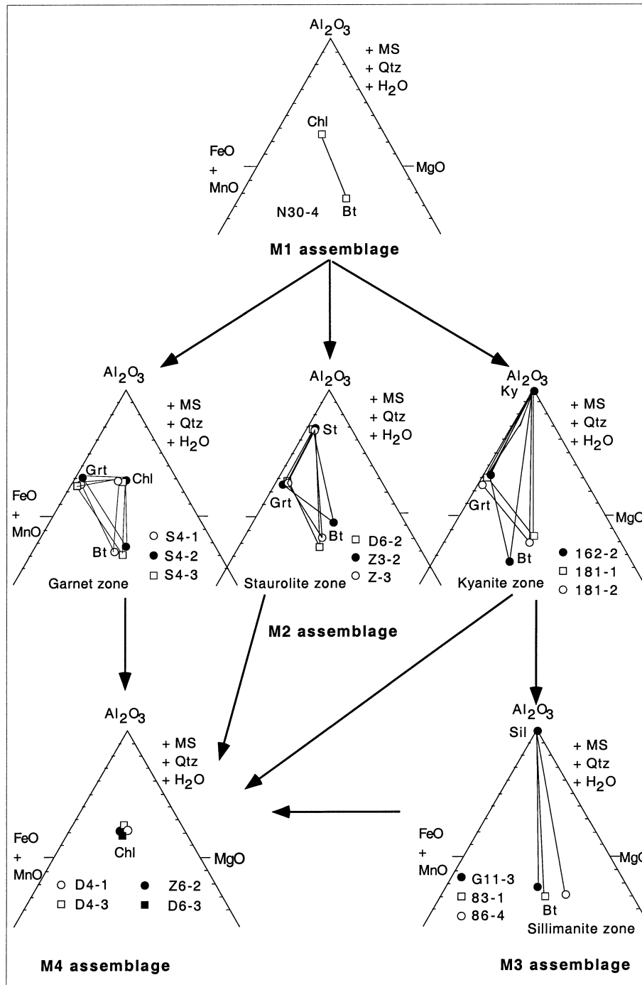
Fig. 6. \text{Al}_2\text{O}_3 –(FeO + MnO)–MgO (AFM) projection of the M1, M2, M3 and M4 mineral assemblages in the Mayuan metapelites. Mineral symbols are after Kretz (1983).
