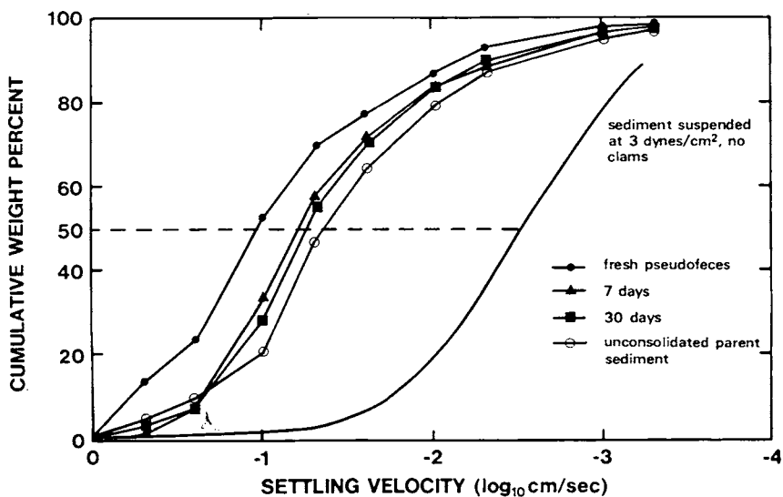
Fig. 7. Settling velocity (size) distribution of parent sediment and clam pseudofeces incubated for various amounts of time.
