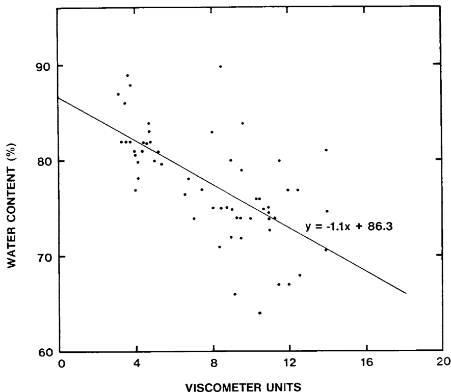
Fig. 3. Regression of water content of laboratory sediment on viscometer torque. T bar length = 3.65 cm, diameter = 0.07 cm. Rotation rate = 10 RPM One viscometer unit \approx 575 ergs.
