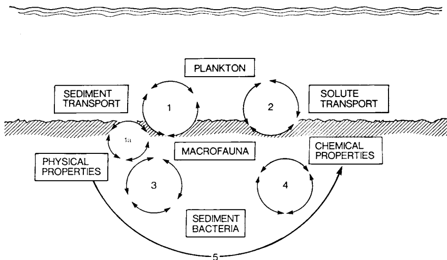
Fig. 1. Schematic depiction of animal-sediment-water interactions in muddy sediments.
