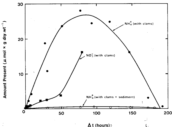
Fig. 12. Amount of nitrate and ammonium in water overlying clams and clams plus sediment. Control values of \text{NH}_4^+ and \text{NO}_3^- in deionized water above are near zero and constant for 200 hrs. Clam excretion was taken to be the sum of darkened circles and squares for the first 50 hrs.
