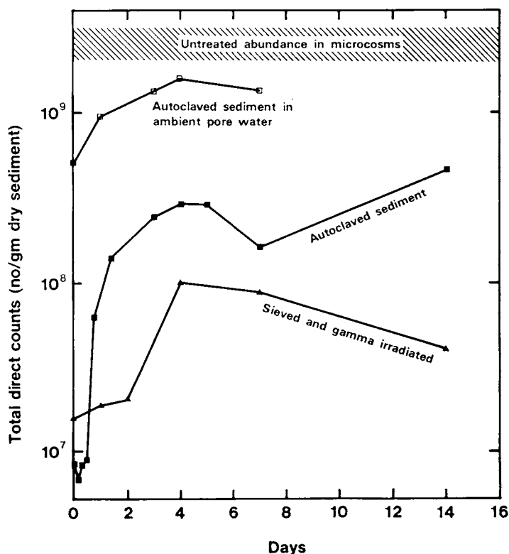
Fig. 13. Bacterial growth in sterile sediments seeded with different amounts of western Lake Erie sediment.
