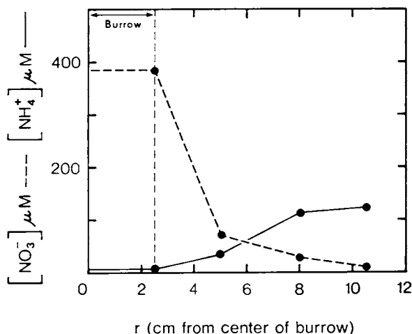
Fig. 9. Nitrate concentrations (dashed line) and ammonium concentrations (solid line) in the 0 to 2 cm interval of the cores plotted as a function of radial distance from the center of the clam burrow.
