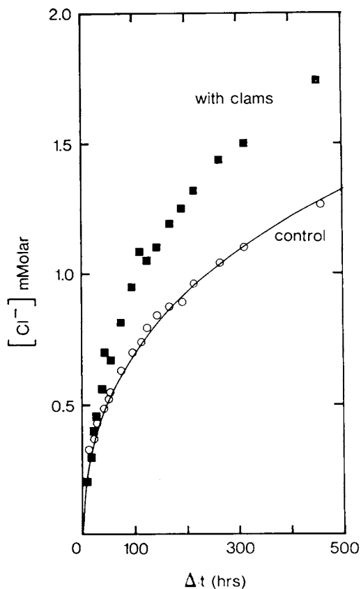
Fig. 10. Chloride concentration in water overlying chloride-spiked sediments with and without clams.
