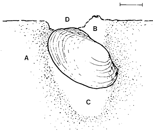
Fig. 2. Typical life position of L. radiata . A = sediment unmixed by burrowing; B, C = zone of complete sediment mixing; D = burrow opening. Scale bar = 2 cm.
