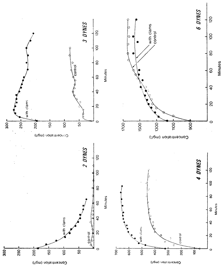
Fig. 5. Entrainment of sediment in the flume with and without Lampsilis .
