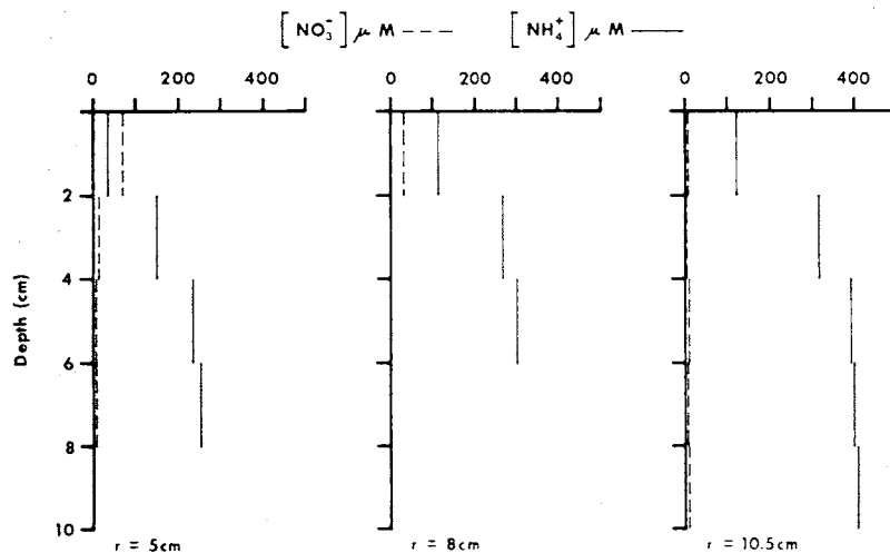
Fig. 8. Pore water nitrate concentrations (dashed lines) and ammonium concentrations (solid line) in sediments containing clams. Profiles are located 5, 8, and 10.5 cm from the center of a clam burrow (2.5, 5.5, and 8.0 cm from the burrow wall).
