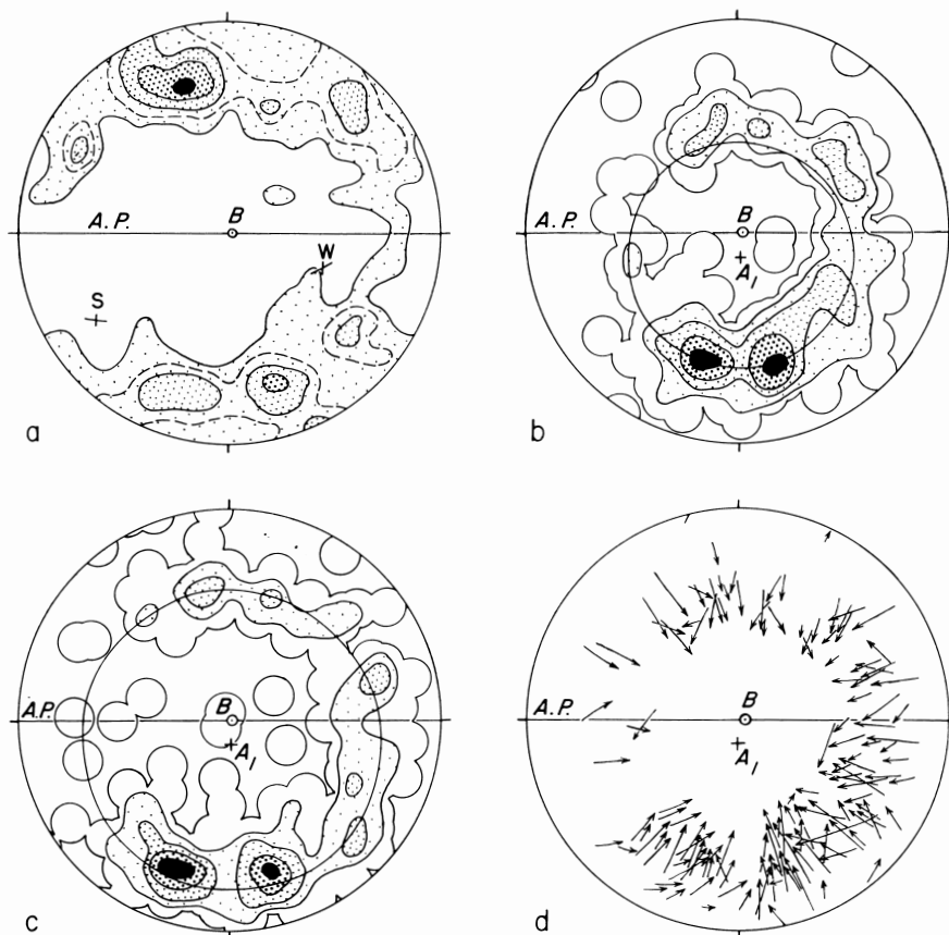
Fig. 2. Orientation data for specimen I.
