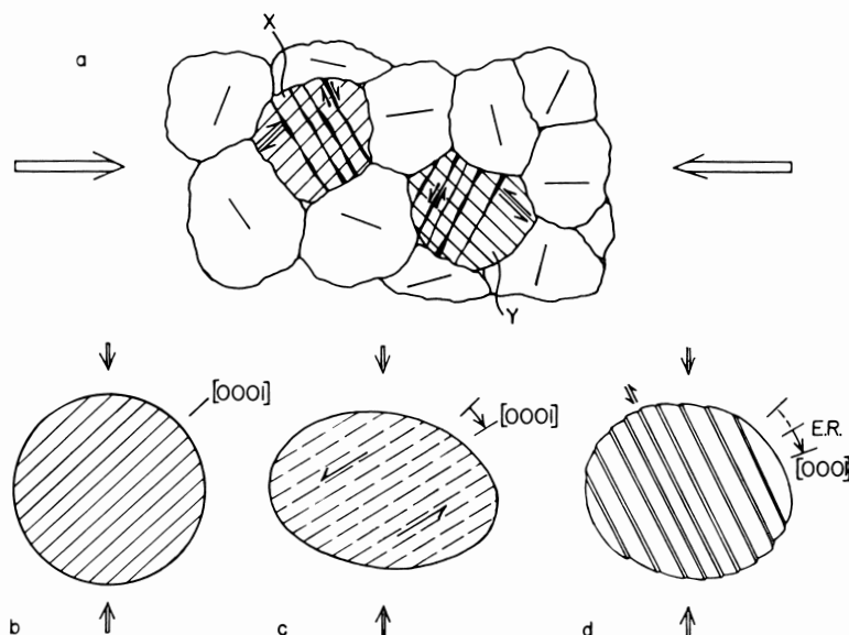
Fig. 7. Diagrammatic representation of the process of formation of deformation lamellae.
