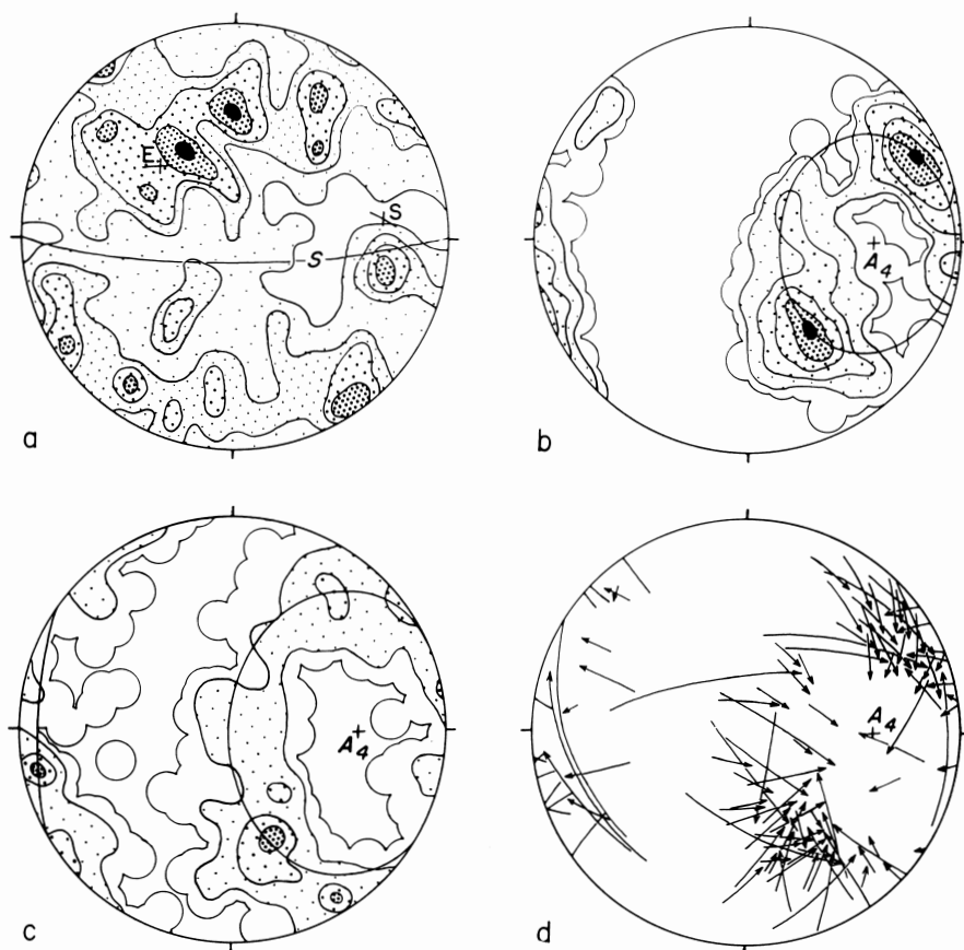
Fig. 5. Orientation data for specimen IV.
