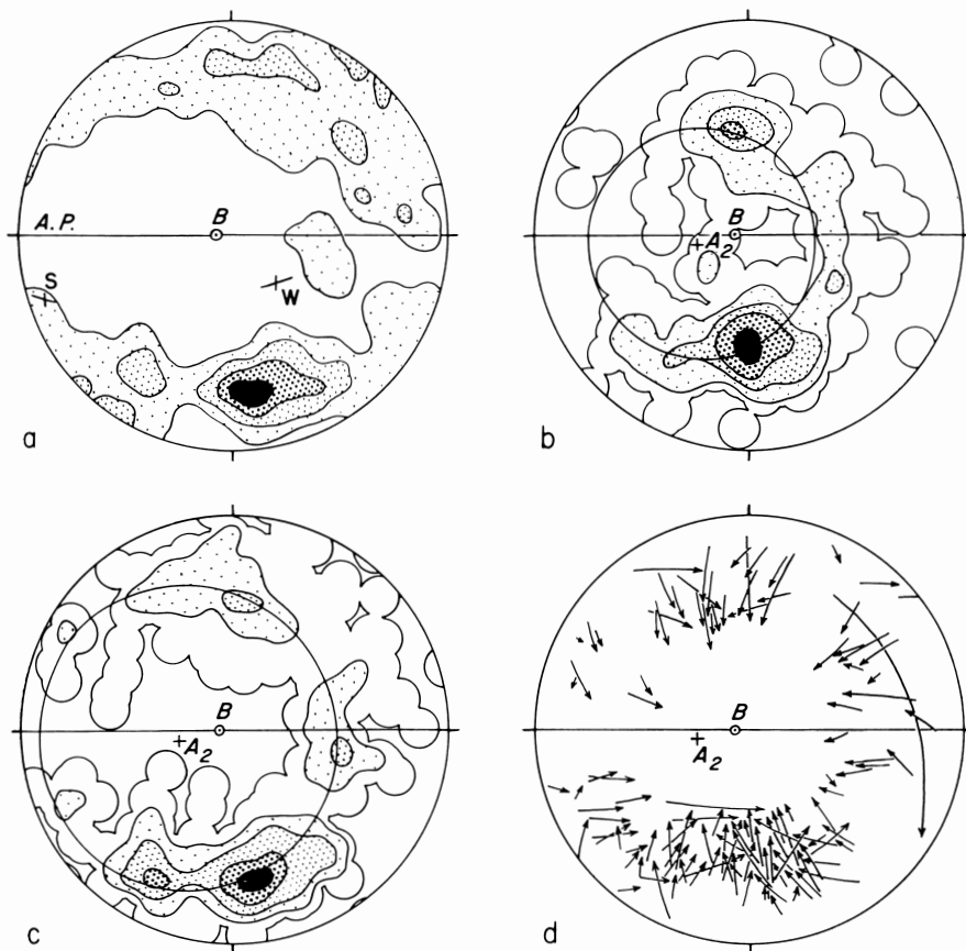
Fig. 3. Orientation data for specimen II.
