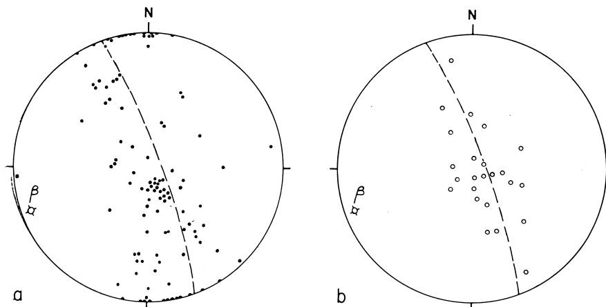
Fig. 8. Data from the Baraboo Quartzite (after Riley, 1947). a. Poles of planar structures (bedding, shear-surfaces, etc.) in the Baraboo syncline. \beta represents the regional fold-axis. b. Compression axes ("a-axes" of Riley) deduced from the orientation of deformation lamellae in specimens of the Baraboo Quartzite. In both diagrams the primitive circle is horizontal with north (N) at the top.
