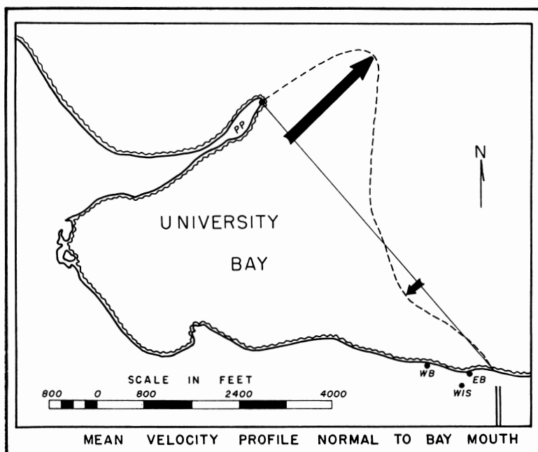
Fig. 2. Mean current profile normal to bay mouth at 1 meter depth. Transport per 10,000 seconds is shown. PP indicates Picnic Point.
