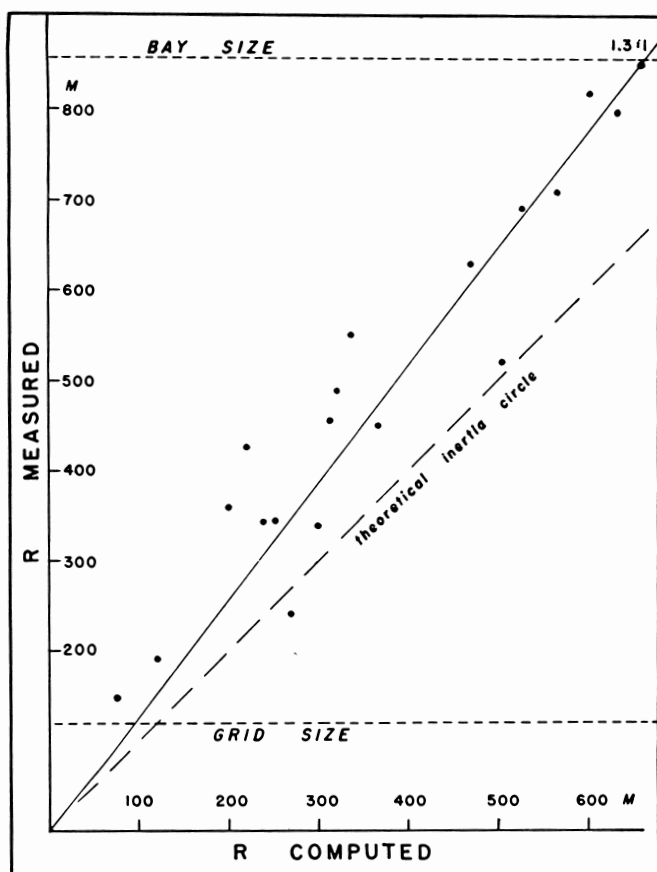
Fig. 5. Computed radius of inertia circle with velocity given by maximum outflow and inflow versus measured radius (i.e. half the distance between regions of maximum outflow and inflow).
