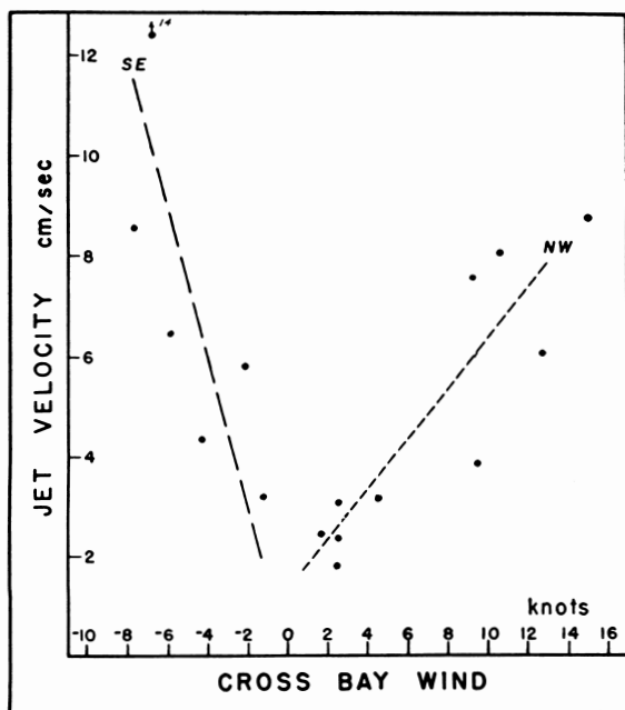
Fig. 4. Cross-bay wind component versus jet velocity relative to mean current. 1 meter depth. Wind as in figure 1.
