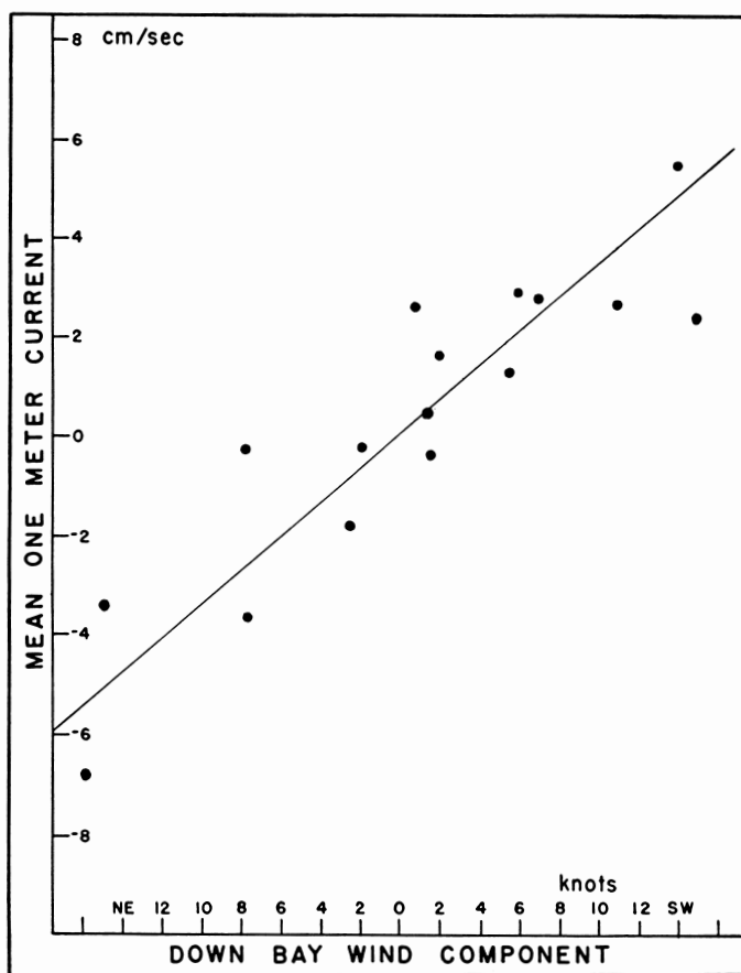
Fig. 1. Down-bay wind component versus mean 1 meter current. The winds were measured at Truax Field near Lake Mendota, but are probably representative for the lake.
