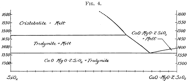
FIG. 4.—The binary system SiO 2 -CaO.MgO.2SiO 2 , wt. per cent.
