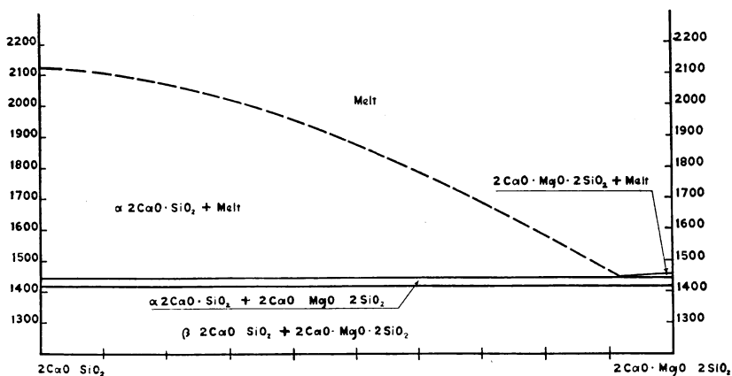
FIG. 16.—The binary system 2\text{CaO}.\text{MgO}2\text{SiO}_2\text{-}2\text{CaO}.\text{SiO}_2 . wt. per cent.
