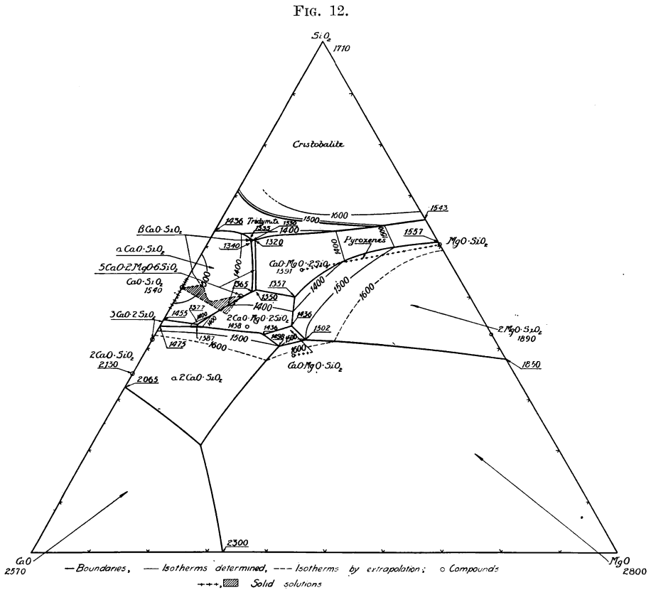
FIG. 12.—A concentration diagram somewhat similar to that given in fig. 8 upon which the isotherms showing the temperatures of complete melting of the various compositions are drawn. The diagram is on a wt. per cent basis.
