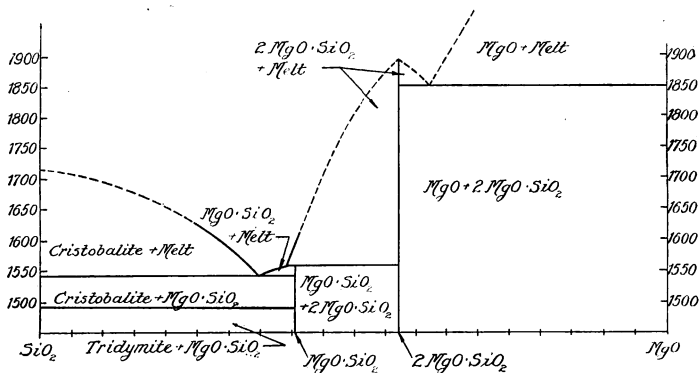
FIG. 3.—The binary system MgO-SiO 2 , weight per cent.
