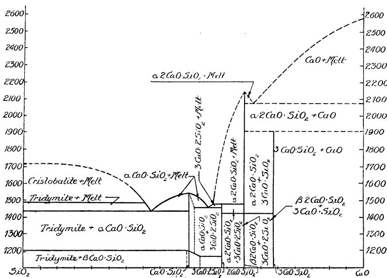
FIG. 2.—The binary system CaO-SiO 2 , weight per cent.
