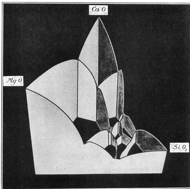
FIG. 9.—A model constructed by plotting vertically upon the concentration diagram as given in fig. 8, the temperature of complete fusion of the boundaries of the fields of stability of the various phases.
