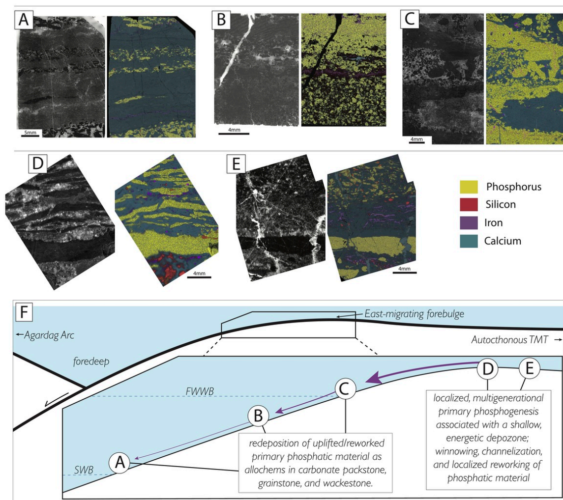
Figure 13. Kheseen Fm. phosphorite facies, presented as a thick-section photograph (left) and micro-XRF-derived elemental map (right). A) phosphatic allochems within grainstone horizons in interbedded limestone grainstone and mudstone. B) fining upward grainstone predominantly composed of phosphatic grains, with infrequent void-filling micritic cement. C) cross-bedded phosphatic wackestone and limestone grainstone. Note variably angular phosphatic clasts in coarsest wackestone horizon. D) Phosphatic hardground and overlying intraclast breccia, with tabular phosphatic clasts supported in a limestone grainstone matrix. Note siliceous cementation of limestone grainstone below basal phosphatic hardground. E) Phosphatic hardground, below limestone grainstone and wackestone with angular phosphatic and chert allochems. F) cartoon schematic model of the Kheseen Fm. phosphogenic sedimentary environment. The putative depositional environments of phosphorite facies A-E are shown, with predominantly-reworked facies (A-C) occurring at or below fair-weather-wave base (FWWB), and likely above storm-wave base (SWB). Facies D and E are indicative of primary, multigenerational phosphogenesis in a shallow, energetic environment, likely on a banktop/local topographic high. The development of locally-variable topography was likely mediated by the eastward migration of a forebulge associated with the collision of the Agardag Arc.
