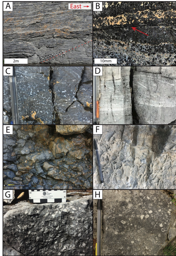
Figure 5. Field photographs of Khuvsgul Group strata. A) Outcrop-scale photograph of well-bedded mudstone-grainstone parasequences of the Salkhitai Mb of the Bakh Fm near Agariin Gol. White dashed lines highlight bedding planes through a m-scale fold, with elongated west-dipping fold arms indicating top-to-the-east shear. The trend of the fold axis highlighted by the red dashed line is parallel to the trend of D1 structures in the Khoridol Saridag Range. B) phosphatic grainstone of the Kheseen Fm, featuring truncated bedding as well as horizons indicative of primary/multigenerational phosphogenesis. The red arrow indicates the location of a multigenerational phosphogenic horizon (phosphatic allochems in authigenic CFA cement). C) thrombolytic texture in a phosphatic grainstone interval of the Kheseen Fm. D) imbricate, edgewise breccia horizon within the Kheseen Fm, featuring rip-up clasts of underlying strata. E) wildflysch of the upper Kheseen Fm at Kheseen Gol. Clasts include material similar to underlying Kheseen strata, suggesting an erosive contact at the base of the interval. F) digitate stromatolites in a dolomite grainstone interval of the Middle Mb of the Erkhelnuur Fm. G) bed-penetrating ichnofossils in a limestone grainstone bed of the Middle Mb of the Erkhelnuur Fm. H) disassociated archaeocyathid allochems in a dolomite grainstone bed of the Upper Mb of the Erkhelnuur Fm. The mechanical pencil in panels C-F and H is 15.5 cm in overall length.
