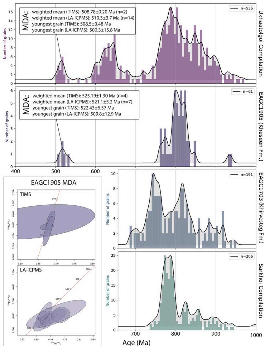
Figure 9. Detrital zircon age spectra from the Khuvsgul study area arranged by relative stratigraphic height. Upper inset panels show maximum depositional age (MDA) constraints for the Kheseen Fm (EAGC1905) and the Ukhaatolgoi Fm (compilation of multiple samples) respectively, as determined by the youngest grain and youngest population of zircon analyzed by both CA-ID-TIMS and LA-ICP-MS. Lower left inset: concordia diagrams for CA-ID-TIMS and LA-ICP-MS analyses of the youngest grains in EAGC1905. All sample locations and geochronological data are compiled in the Supplementary Information (table S3).
