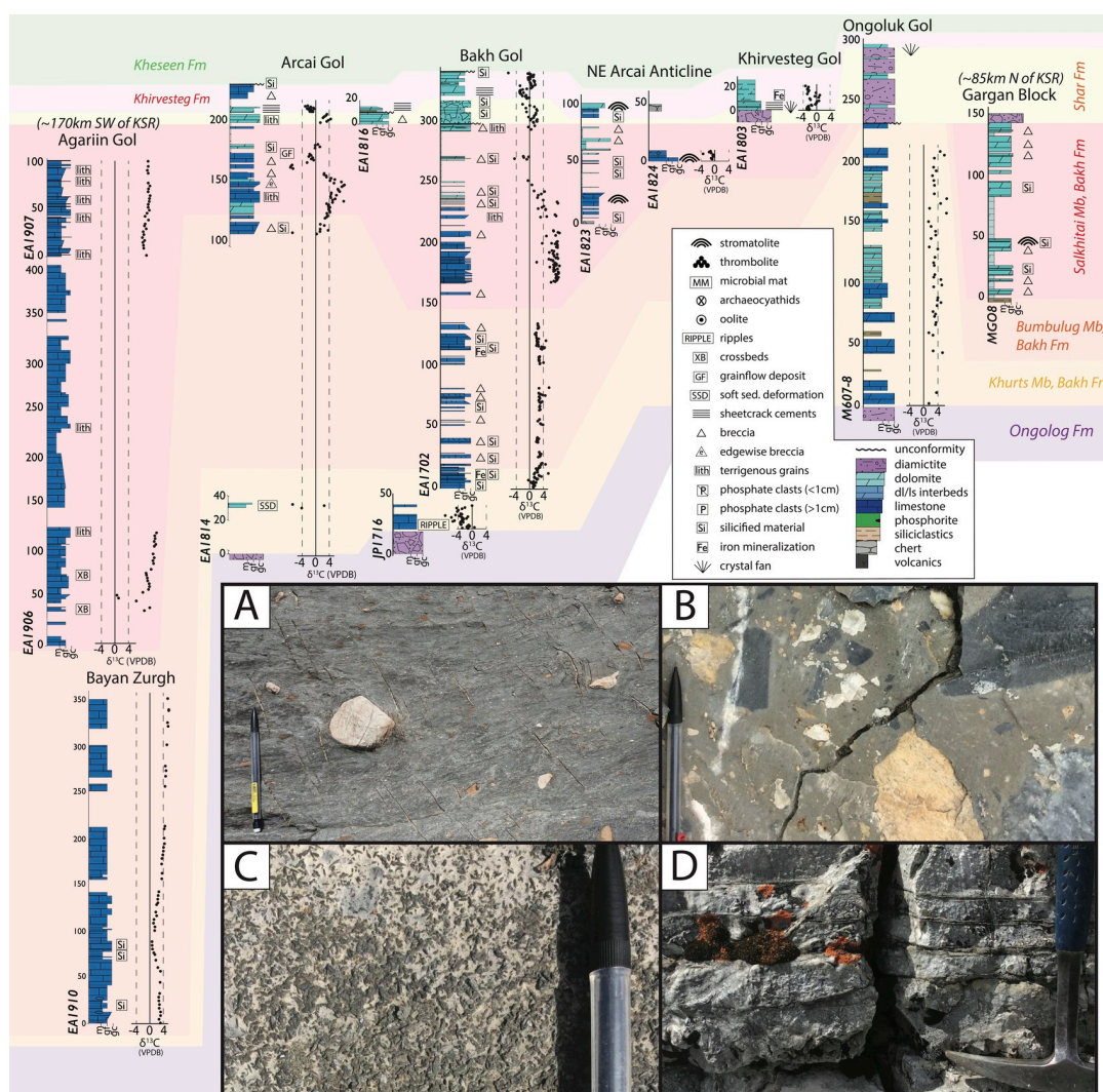
Figure 4. Cryogenic chemostratigraphy of the Khuvsgul Group, with field photographs of Cryogenic lithologies depicted in inset panels A-D. Stratigraphic sections are arranged, from left to right, along a broadly southwest-northeast transect. Geochemical data and section locations are collated in the Supplementary Information (tables S1, S3). A) massive, matrix supported diamicrite of the Ongolog Fm. B) massive diamictite of the Shar Fm, featuring carbonate clasts in a dolostone matrix. C) barite pseudomorphs on a dolomite grainstone bedding plane in the basal Khirvesteg Fm. D) sheetcrack cements in dolomite mudstones of the basal Khirvesteg Fm. The mechanical pencil in panels A–C is 15.5 cm in overall length; the hammer in panel D is 33 cm long overall.
