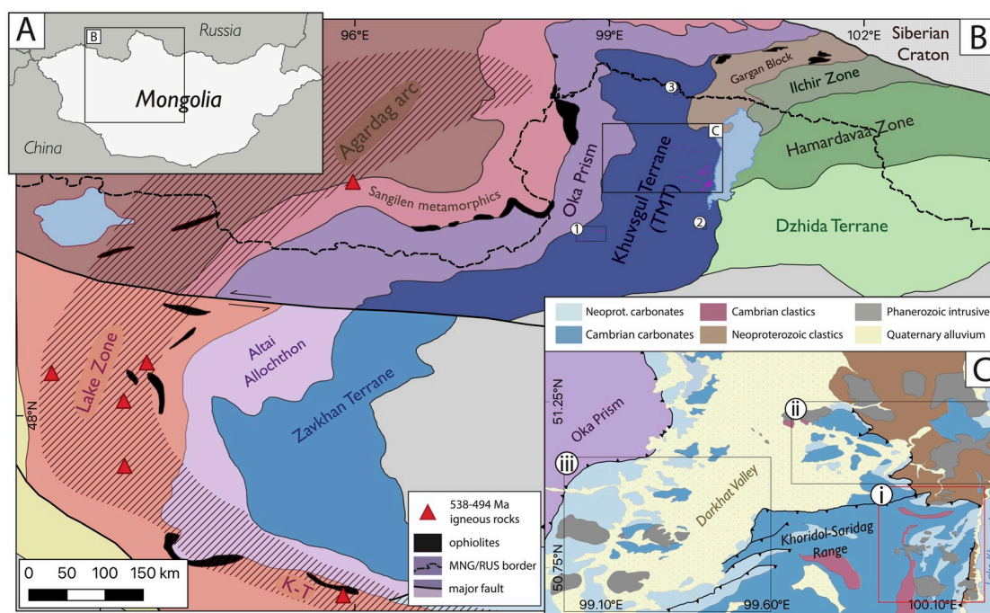
Figure 1. Location and geological context of study area: A) geopolitical overview map, contextualizing B) the Mongolian Central Asian Orogenic Belt, modified from Bold, Crowley et al. (2016), Bold et al. (2019), and Kuzmichev (2015). The Khuvsgul Terrane forms the core of the composite Tuva-Mongolia Terrane (TMT). The location of 538–494 Ma igneous rocks, as well as the hashed area indicating the putative extent of the Ikh-Mongol continental arc, are modified from Janoušek et al. (2018). The numerals 1, 2, and 3 indicate the positions of the Bayan Zurg, Eg Gol, and Khoroo Gol study areas, respectively. C) Generalized geologic map of the main Khuvsgul study area, compiled from both original and extant geological mapping (Buihover et al., 1968). Boxes with numerals i, ii, and iii indicate the extent of the Khoridol Saridag, northern, and Darkhat Valley mapping regions, respectively. A 1:100,000 geological map of the Khoridol Saridag mapping area can be found in figure 3 ; geologic maps of the Northern and Darkhat Valley mapping areas can be found in the Supplementary Information.
