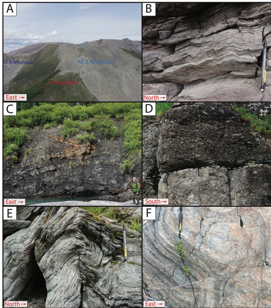
Figure 8. Field photographs detailing structural elements of the greater Khuvsgul study area. A) a laterally-discontinuous sliver of Ukhaatolgoi Fm sediment forms the footwall of an east-dipping backthrust in the southeast Khoridol Saridag Range. B) crenulation cleavage in a fine-grained lithic wacke of a Sarkhoi Fm outcrop approximately 1 km north of the Arcai Gol Thrust. Elongated cleavage planes, dipping to the south-southwest, indicate shear in a top-to-the-north-northeast direction, consistent with the putative throw of the Arcai Gol Thrust. Primary bedding planes are dipping to the west (broadly into the page). C) chevron folds in the Salkhitai Mb of the Bakh Fm, eastern Darkhat Valley. Approximately 1.7-m-tall geologist for scale. Folds are broadly D1 parallel, and indicate eastward vergence, putatively associated with their proximity to D) cataclasites adjacent to a major east-dipping backthrust (fault surface highlighted with a white dashed line) running along the western margin of the Darkhat Valley and defining the western extent of the Khoridol Saridag Range. E) fabrics representative of those observed in siliciclastic lithologies across the Northern mapping area. F) foliations in granodiorite (EAGC1942) of the northern area are broadly axial-parallel to D1 structures. The mechanical pencil in panels B, E, and F is 15.5 cm in overall length.
