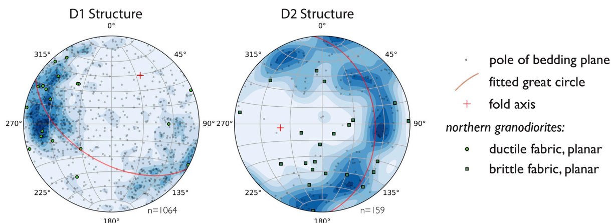
Figure 7. Stereonets showing the orientations of km-scale folds in the Khoridol Saridag Range that are representative of D1 and D2 structures, respectively. Individual bedding measurements are depicted as poles to bedding planes. Ductile fabrics (dominantly folded foliation) observed in granodiorites from the Northern mapping region (including EAGC1942, 1943, and 1944) are shown on the D1 stereonet, while brittle fabrics (dominantly small-scale, cm-offset faults) observed in the same granodiorites are superimposed on the D2 stereonet. D1 structures are interpreted to be coeval with (or marginally postdate) the emplacement of the granodiorites, while D2 structures likely postdate granodiorite emplacement. The map locations of all major D1 and D2 structures in the Khoridol Saridag and northern mapping regions, as well as representative structural measurements, are presented in the Supplementary Information (fig. S1).
