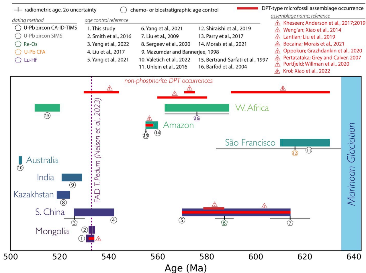
Figure 14. Age and duration of Ediacaran and Cambrian phosphorite occurrences, grouped by craton. The temporal range of Doushantuo-Pertatataka-Type microfossil assemblages, including those not associated with phosphorites, are depicted in red.
