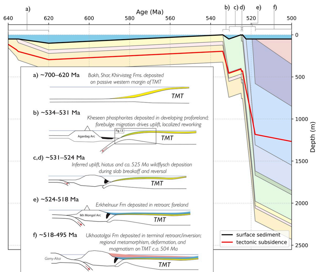
Figure 12. Tectonic subsidence model for the Khuvsgul Group, paired with a schematic tectonic model (inset panel) of the western margin of the Tuva-Mongolia Terrane in Khuvsgul Group time. a) passive margin deposition occurred along the western margin of the TMT during the Cryogenian and early Ediacaran, prior to a prolonged depositional hiatus along the margin. b) deposition of the fossiliferous phosphorites of the Kheseen Fm occurred in a pro-foreland basin associated with the approaching Agardag Arc; see figure 13 for detailed schematic of phosphogenic environment. c,d) collision of the Agardag Arc resulted in slab breakoff and subduction polarity reversal; uplift associated with these events inverted the pro-foreland, caused putative erosion/hiatus, and resulted in the deposition of wildflysch in the eastern Khoridol Saridag Range. e) resumption of E-dipping subduction along the western margin resulted in Ikh-Mongol Arc magmatism, and the deposition of the Erkhelnuur Fm into the Ikh-Mongol retroarc foreland. f) collision along the western margin of the Ikh-Mongol arc resulted in regional metamorphism, inversion of the retroarc foreland, deposition of the Ukhaatolgoi Fm., and the emplacement of granodiorites ca. 504 Ma.
