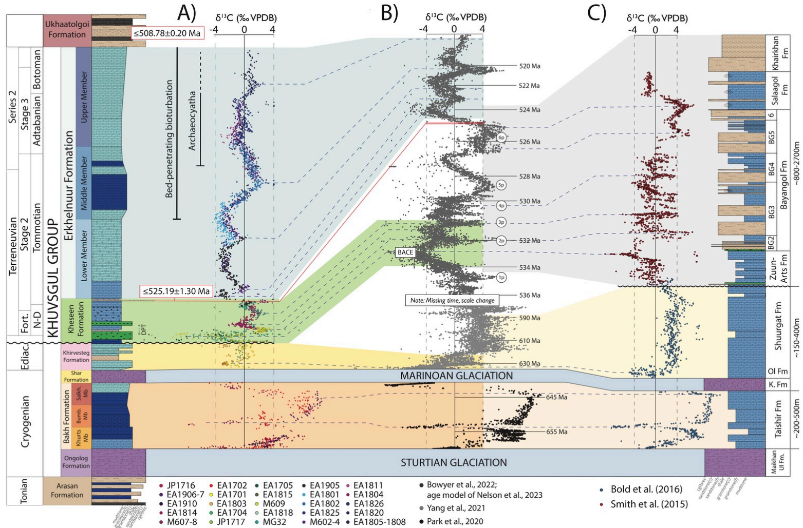
Figure 11. Age model and compiled chemostratigraphy for the Khuvsgul Group. A) a \delta^{13}\text{C} compilation from the Khuvsgul group is correlated with B) a global \delta^{13}\text{C} compilation and C) a composite \delta^{13}\text{C} chemostratigraphy from Cryogenian-Cambrian strata of the Zavkhan Terrane. Note that while we use the global chemostratigraphic compilation of Bowyer et al. (2022), we utilize the Cambrian age model of L. L. Nelson et al. (2023).
