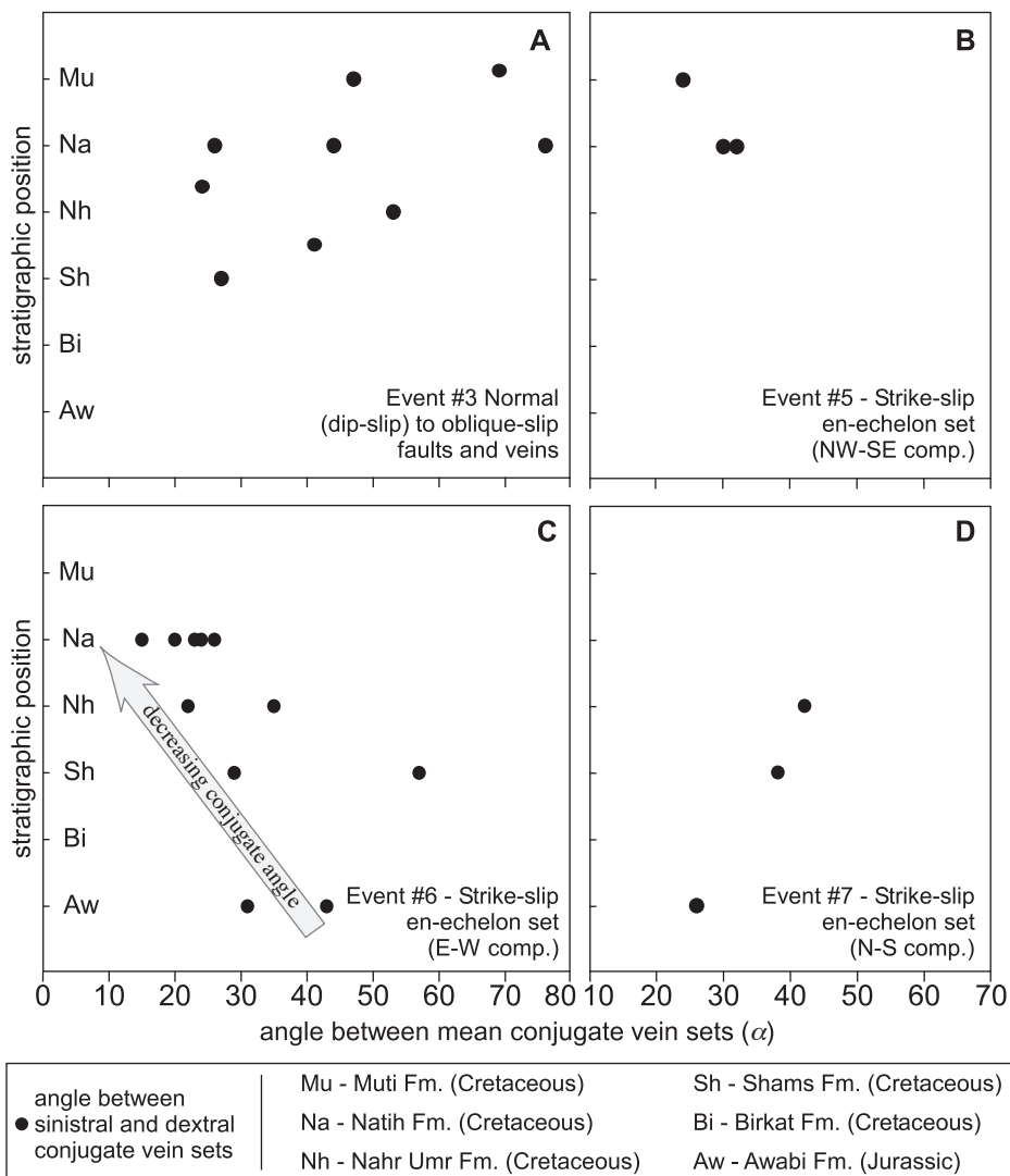
Fig. 15. Graphs showing the acute angles between mean orientations of conjugate sets ( \alpha ) of fractures and veins versus stratigraphic position (related to depth) of the structures (see fig. 2). The data is organized by tectonic events. Note that the only event where there is a significant trend of conjugate angles (hence angle of internal friction or effective fluid pressure) is event #6. In this case conjugate angles ( \alpha ) increase with depth. The lowest values occur at the Natih Fm, just below the Muti Fm. The relative thickness of each formation is not displayed in the graph, so that the Y-axis does not have a scale.
