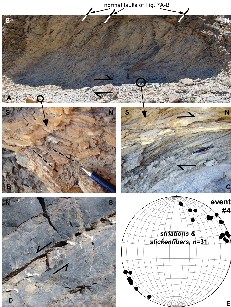
Fig. 9. Effects of event #4. (A) S-N view of top-the-Northeast shearing of the normal faults of figures 7A-7B (Nahr Umr Fm). (B) Detail of layer-parallel striations pointing towards the Northeast. (C) Detail of top-to-the-northeast layer-parallel shearing. (D) Sigmoidal calcite veins sheared towards the NE (Shams Fm). (E) Summary of the orientations of striations and slickenfibers directions at the six localities where layer- and cleavage-parallel veins with a NE shearing direction were found (event #4). Each dot represents the average of measurements at each outcrop. Note that original orientations have been rotated in this plot considering that layers were horizontal when these structures were formed.
