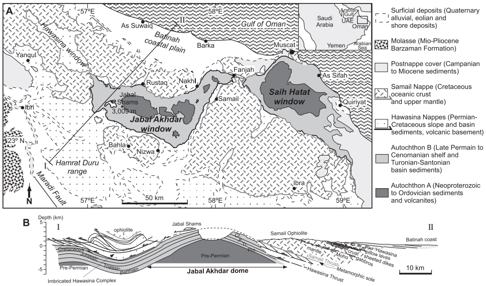
Fig. 1. (A) Geological map of the central part of the Oman Mountains. The Jabal Akhdar and Saih Hatat tectonic windows expose rocks of the Autochthons A and B. (B) NE-SW cross-section. Figure (A) is modified from Breton and others (2004), who compiled it from the Geological Map of Oman, scale 1:1,000,000 (Le Métour and others, 1993). Figure (B) is modified from Searle (2007).
