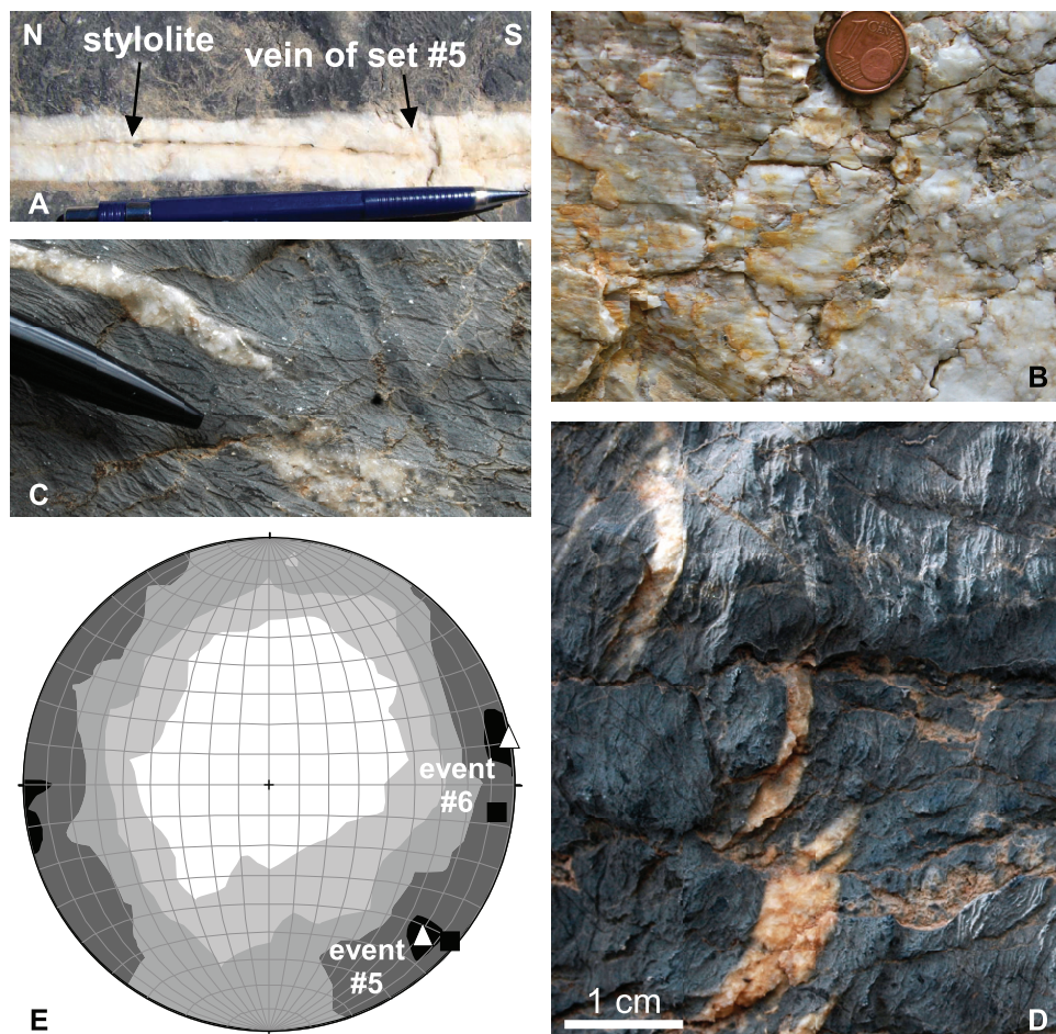
Fig. 11. (A) Detail of a tectonic stylolite (developed during stage #6) dissolving a vein of event #5. (B) Tectonic stylolites dissolving dip-slip and strike-slip striations on a large-scale fault plane. (C) Complex relationships between structures: tectonic stylolite dissolves a calcite vein of event #5 and the same vein crosscuts tectonic stylolites. (D) Bedding-parallel stylolites cutting a vein of event #5. (E) Stereoplot showing the data collected from tectonic stylolites in the southern limb of the Jabal Akhdar area. Figure displays pole plots and Kamb contours indicating two maximum compression directions: NW-SE (event #5) and E-W (event #6). A total of 41 measurements are displayed in this plot. White triangles show the average orientations of \sigma_1 calculated from tectonic stylolites of both sets. For comparison, black squares indicate the average orientations of \sigma_1 for the sets of fractures and veins of events #5 and #6.
