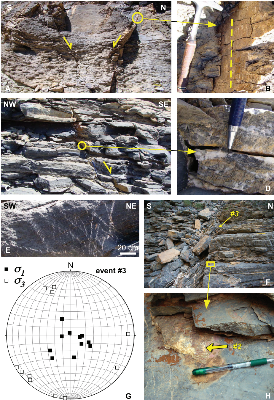
Fig. 7. Structures of event #3. (A) Conjugate normal faults in the Nahr Umr Fm. (B) Detail of vertical striations on the right normal fault of photo (A). (C) One set of normal faults filled with calcite in limestones of the Shams Fm. (D) Detail of vertical striations on fault plane of photo (C). (E) View of an outcrop in the Natih Fm with conjugate sets of en-échélon and sigmoidal veins formed due to a \sigma_1 perpendicular to layers (that is, subvertical). (F) Normal fault (event #3) offsetting a layer-parallel vein with a top-to-S sense of shearing (event #2). (G) Summary of the orientations of principal compression stresses \sigma_1 and \sigma_3 at the localities where these structures were found. Each square represents the average of measurements at each outcrop. Note that the original orientation data have been rotated in this plot assuming that layers were horizontal when these structures formed. (H) Detail of photo (F).
