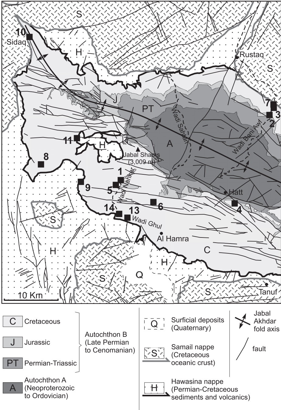
Fig. 3. Simplified map of the western part of the Jabal Akhdar dome. Squares with numbers indicate the location of the areas used for this study. Dashed lines are rivers or water streams that define wadis (valleys). A complete list of localities with coordinates is shown in table 1. Figure compiled from the Geological Map of Oman (Rustaq sheet), scale 1:100,000 (Beurrier and others, 1986). Locality 12 is out of the map. Thin lines indicate fault traces. The geographical coordinates of the upper left corner are (57°00'E, 23°30'N).
