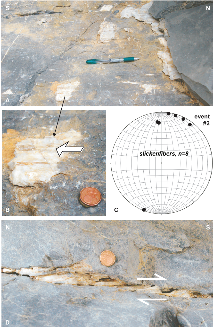
Fig. 6. Structures of event #2. (A) Slickenfibers on shallow-dipping veins indicating top-to-the-South sense of layer-parallel shearing in limestones. (B) Detail of photo (A). The diameter of the 1-cent Euro coin is 16.25 mm. (C) Summary of the orientations of slickenfibers on layer-parallel veins at the three localities where they were found. Each dot represents an individual measurement. Note that the original data have been rotated in this plot assuming that layers were horizontal when the structures developed. (D) Stepped layer-parallel vein showing top-to-South movement.
