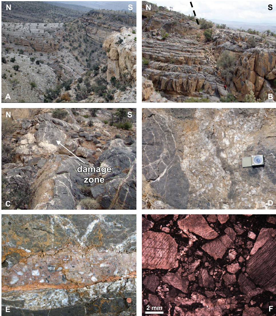
Fig. 8. Structures of event #3, probably reactivated by younger events (#5, #6, #7). (A) Large-scale dip-slip fault with a stratigraphic offset of ~700 m. (B) Large-scale dip- to oblique-slip fault that was later reactivated as strike-slip. (C) The damage zones of some of these faults are containing numerous calcite veins, probably formed during subsequent strike-slip events. (D-E-F) Details of breccias found in the damage zones of one of these large-scale faults. In photo (E), which is oriented W-E, a tectonic stylolite is dissolving the interface between the breccia and the host rock, indicating that the breccia formed before the stylolite. (F) Microphotograph of the fault breccia, taken under plane polarized light.
