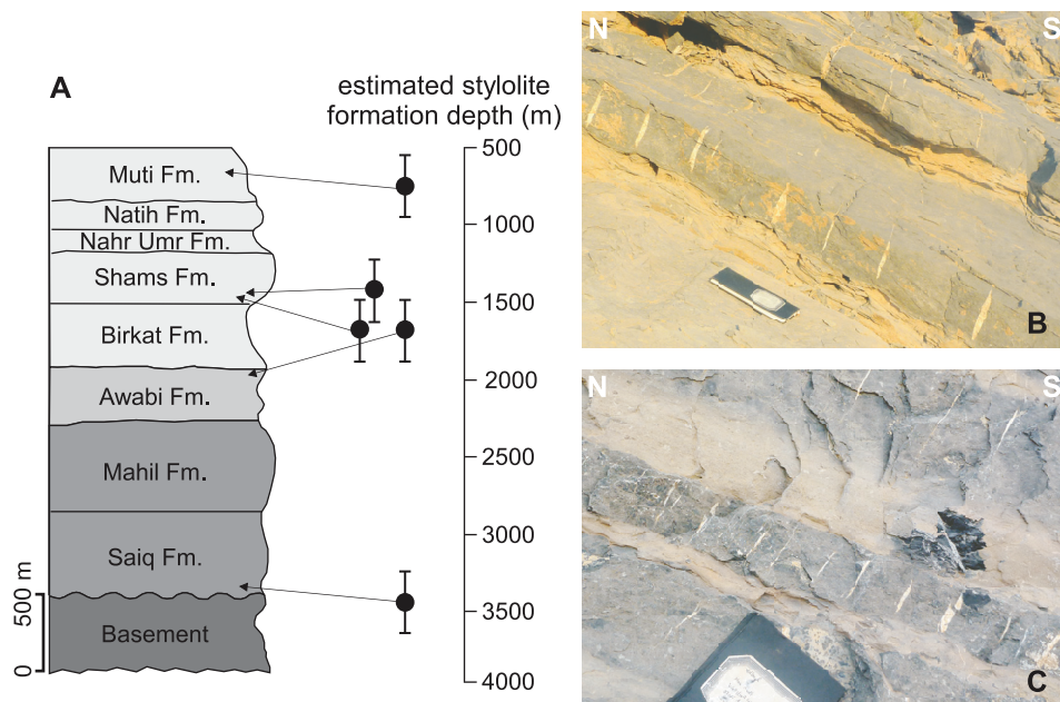
Fig. 5. Structures of event #1. (A) Plot summarizing formation depth of sedimentary stylolites. Arrows point towards the stratigraphic position and unit from where they were collected. (B) Bedding-confined calcite veins with lenticular shape in cross-section. (C) Calcite-filled veins confined to dm-scale beds. Both images show rocks of the Natih Fm. These veins are consistently rotated with bedding due to top-to-the-South thrusting event, which corresponds to event #2. Photographs (A) and (B) were taken at locality 13, and locality 14, respectively.
