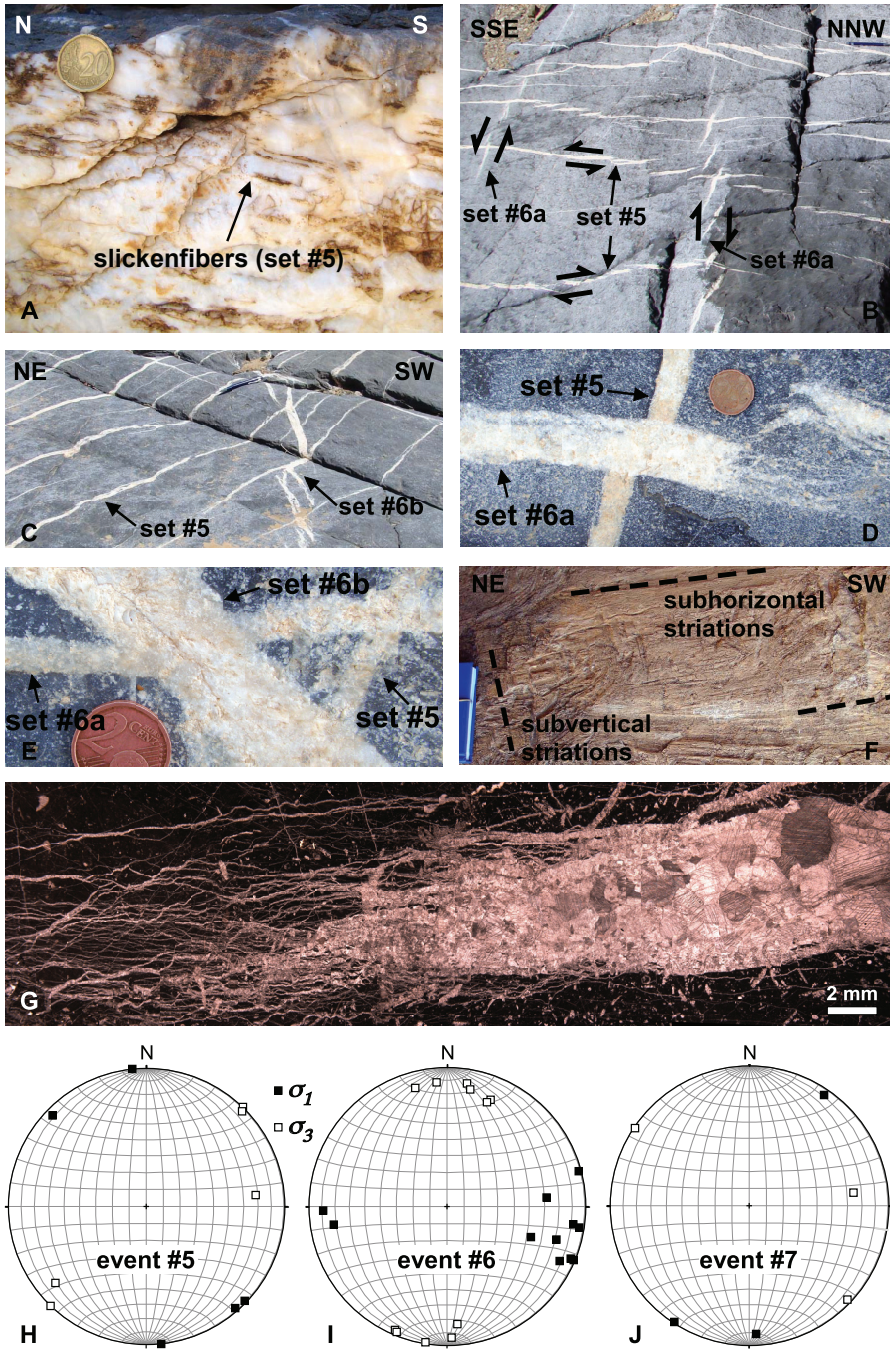
Fig. 10. (A) Vein of event #5 with subhorizontal slickenfiber crystals. (B) En-echelon conjugate sets of veins of event #6a (E-W-compression oriented) crosscutting veins of event #5 (NW-SE-compression oriented). (C) En-echelon veins of event #6b (NNE-SSW-oriented compression) crosscutting veins of event #5. (D-E) Examples of cross-cutting relationships between the different strike-slip vein sets. A stylolite dissolves the center of a vein of event #6b. (F) E-W-oriented large-scale fault with two sets of striations indicating older dip-slip and younger strike-slip movements. (G) Microphotograph showing the typical crack-seal microstructures of veins of the three strike-slip events. These veins are generally formed by hundreds or thousands of
