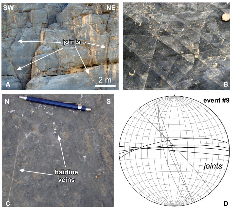
Fig. 12. (A, B) Sets of joints of different scales in the Natih Fm. (C) Thin and straight veins in the Natih Fm. (D) Orientations of joints and associated thin veins. Each great circle represents the average orientation calculated at one outcrop. These orientations are compatible with the present-day stress field in Oman.
