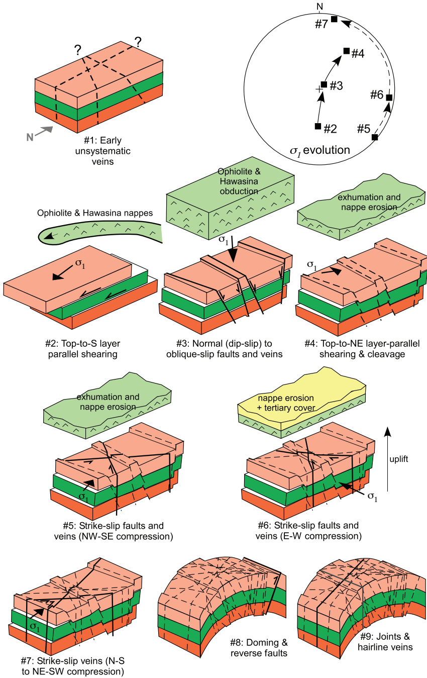
Fig. 13. Sketches summarizing the structural evolution of the Jabal Akhdar dome, with the order of identified events and calculated stress field orientations. The stereogram illustrates the evolution of \sigma_1 showing two main trends: firstly obduction (#2), normal (dip-slip) and oblique-slip faulting (#3), reverse thrusting and exhumation (#4), and secondly a far horizontal \sigma_1 that comprises three events (#5 to #7). It is possible that event #3 did not form after obduction but before it.
