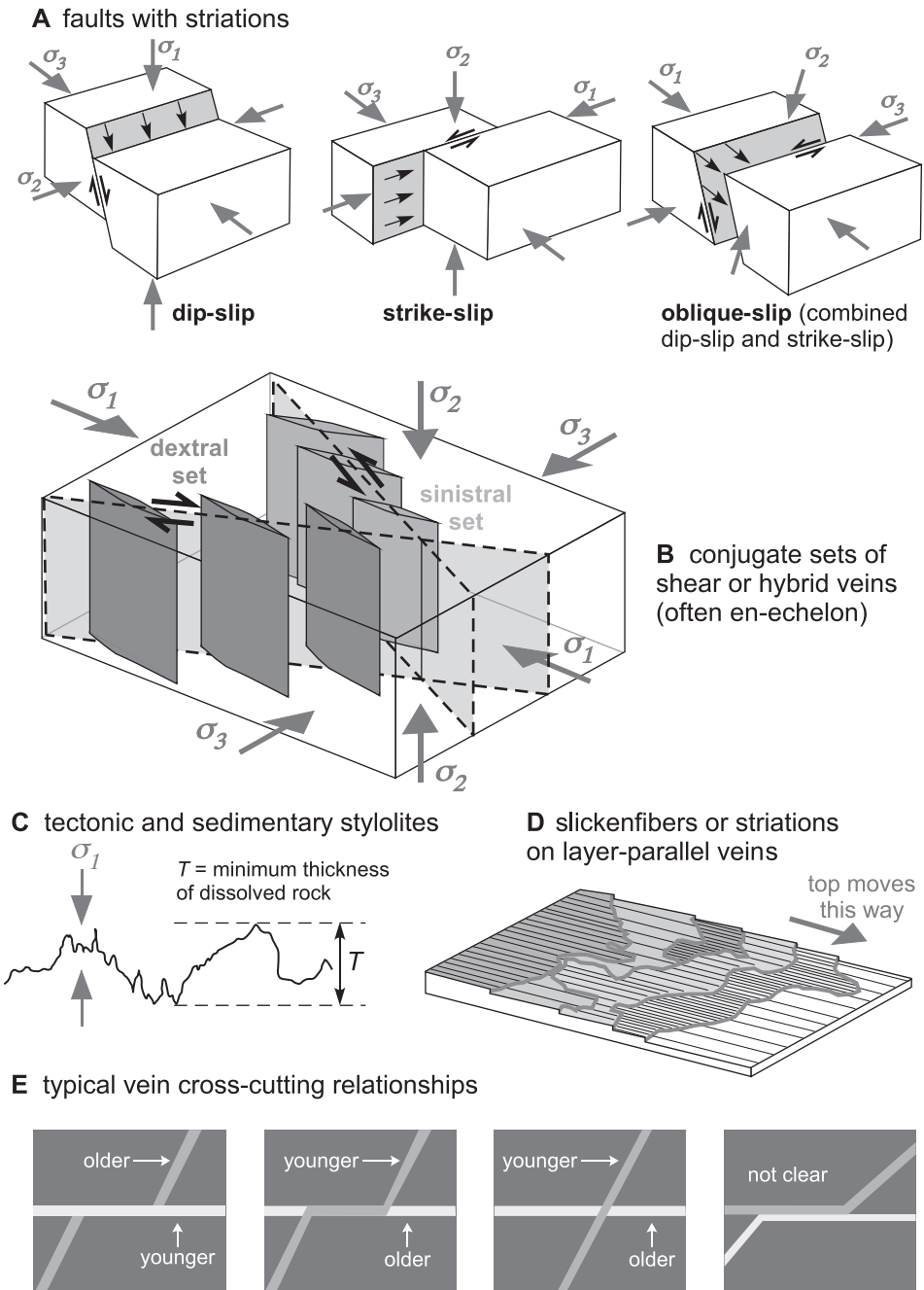
Fig. 4. Sketches summarizing the methods to estimate stress orientations from different structures. (A) Faults with striations (dip-slip, strike-slip and oblique-slip). (B) Conjugate sets of hybrid or shear veins. (C) Tectonic stylolites. (D) Slickenfibers or striations on layer-parallel veins. (E) Sketches showing the typical vein cross-cutting relationships found in the field (for example, Virgo and others, 2013b).
