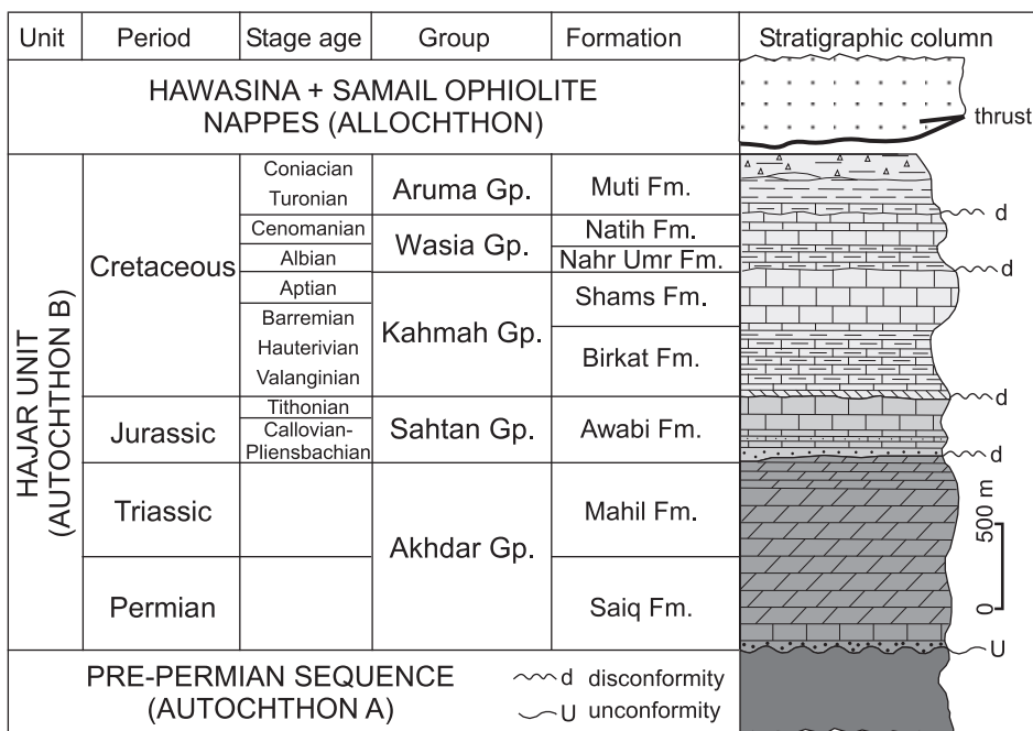
Fig. 2. Simplified lithostratigraphic column of the Autochthonous B units of the Jabal Akhdar area. The log is modified from the Geological Map of Seeb, scale 1:250,000 (Béchenec and others, 1992). The ages of the formations are from figure 2 of Breton and others (2004).
