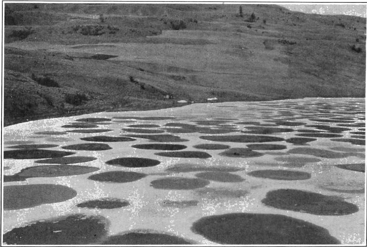
FIG. 1.—Large spotted epsomite lake in British Columbia, on Kruger Mountain. Photograph taken during the dry season in July, 1917.
