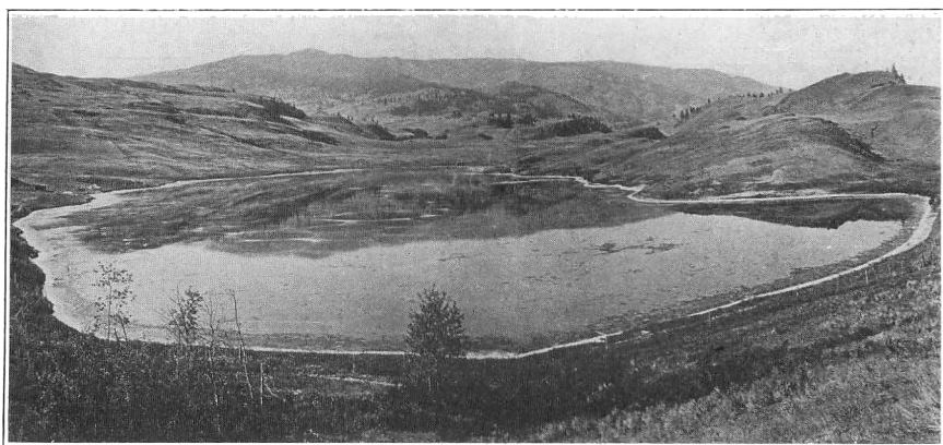
FIG. 5.—Same spotted lake as that in fig. 1. This photograph was taken after the rainy season.
