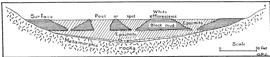
FIG. 4.—Hypothetical vertical cross-section to show structure of small epsomite lake north of Oroville, Washington.
