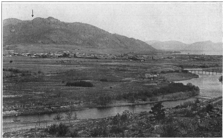
FIG. 3.—View of Oroville with Osoyoos Lake at the right, Okanogen River in the foreground, and Kruger Mountain in the background, with arrow pointing to situation of the small epsomite lake shown in fig. 2.
